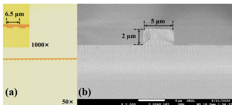
Figure 10. (a) Morphology of actual waveguide gratings measured by optical microscope (50 \times and 1000 \times ) and (b) cross-section of input channel waveguide measured by SEM.
