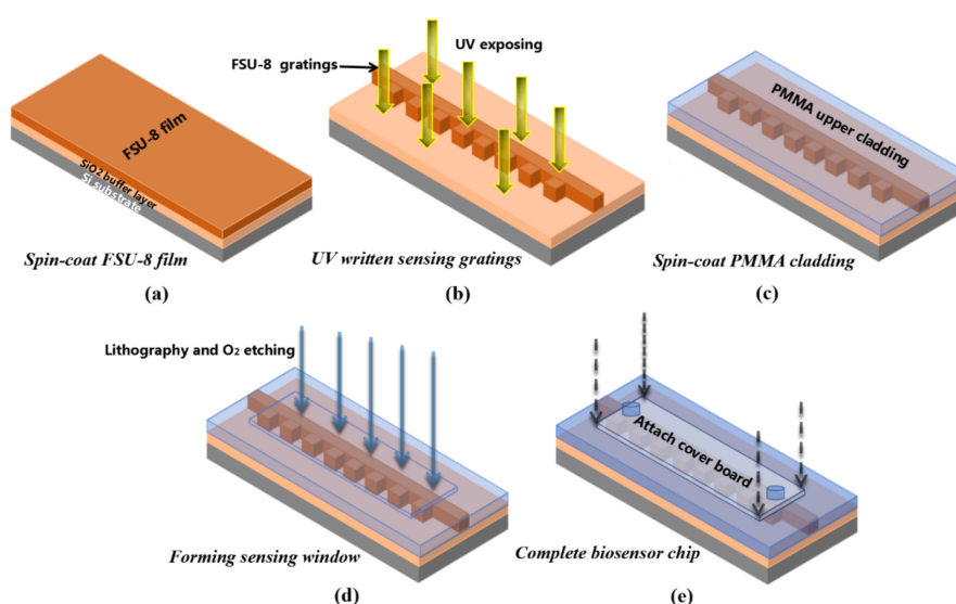
Figure 8. Fabrication process of polymer grating-based biosensor. (a) Spin-coat FSU-8 film, (b) UV written sensing gratings, (c) spin-coat PMMA cladding, (d) forming sensing window, and (e) complete biosensor chip.
