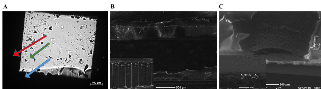
Figure 5. Microscope image of printing results. (A) An area of prints under the microscope. The red, blue, and green arrows indicate graphene, copper tape, and polyimide (PI), respectively, after the annealing process. (B,C) SEM images of printed graphene on PI using 2–5 kV accelerated voltage. (B) is a top-view image taken using SEM after annealing the prints with an average width of \approx 868\text{ }\mu\text{m} . (C) shows an image of a cross section with an average depth of 5.20 \mu\text{m} .
