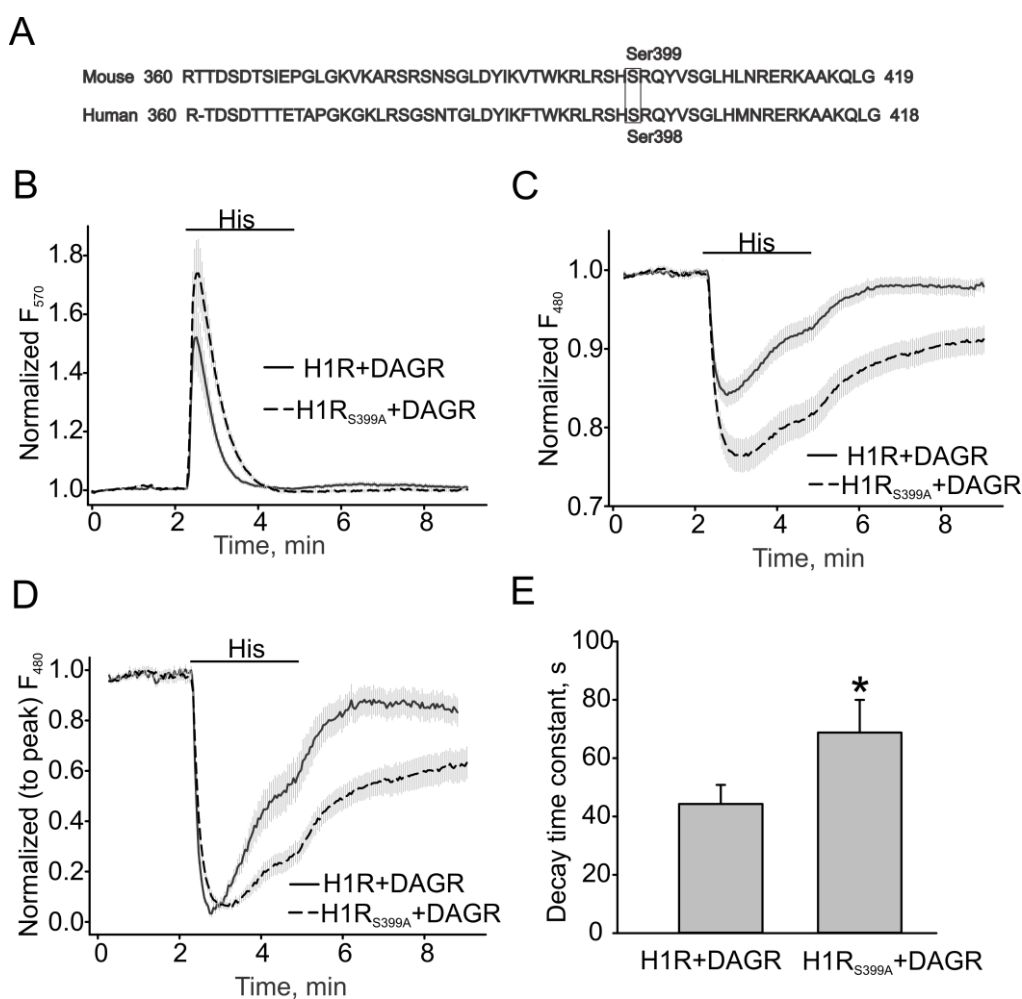
Figure 3. DAG production is more sustained in H1R S399A -expressing HEK cells. (A) Amino acid sequences and PKC phosphorylation sites in human and mouse H1 receptors. (B) \text{Ca}^{2+} changes in H1R and H1R S399A expressing HEK cells. The downward DAG+R-GECO sensor (DAG/ \text{Ca}^{2+} R) was excited at 570 nm for detecting intracellular \text{Ca}^{2+} transients. (C) DAG transients assessed with the downward DAG + R-GECO sensor excited at 480 nm. (D,E) Summary data on the decay time constants for DAG transients. The bold and broken lines represent the averaged traces, and the vertical gray lines are the SEM values. Averaged traces in H1R and H1R S399A expressing HEK cells are shown as solid and broken lines. Data in (E) are presented as mean \pm S.E. Asterisk = p < 0.05 .
