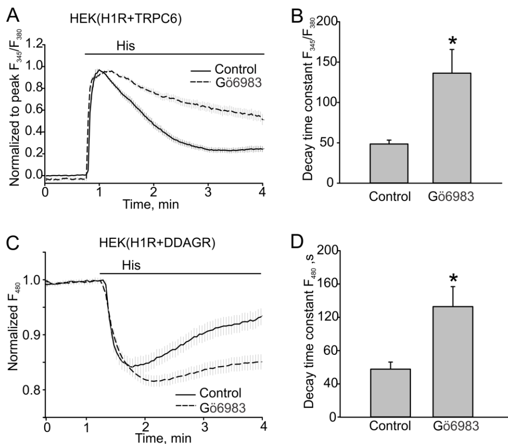
Figure 2. PKC inhibitor G \ddot{ö} 6983 slowed the decay of \text{Ca}^{2+} and DAG signals in the HEK model. (A,B) Histamine-induced \text{Ca}^{2+} transients in HEK cells expressing H1R + TRPC6 in the absence or presence of PKC inhibitor G \ddot{ö} 6983 (500 nM). Fura-2 fluorescence ratios ( F_{345}/F_{380} ) are shown. (A) Traces of averaged \text{Ca}^{2+} transients in the control group and cells treated with G \ddot{ö} 6983 (control, n = 41 vs. G \ddot{ö} 6983, n = 39 ). The ratio data were normalized to the peak amplitude following the baseline fluorescence ratio at time zero was subtracted. (B) Summary data comparing the decay time constants for the \text{Ca}^{2+} transients shown in (A). (C,D) DAG transients assessed with the downwards DAG+R-GECO sensor excited at 480 nm. The fluorescence was normalized to the baseline fluorescence. The bold and broken lines represent the averaged traces, and the vertical gray lines are the SEM values. Data in (B,D) are presented as mean \pm S.E. Asterisk = p < 0.05 .
