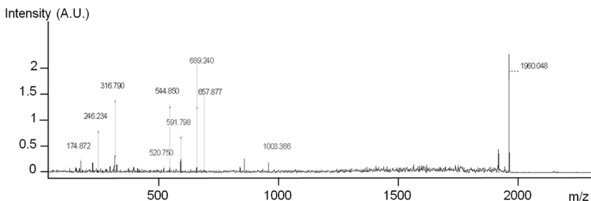
Figure 9. MS 2 analysis of the 1960 Da peak on GaAs (100) functionalized with 10% MHDA after Rat Serum Albumin (RSA) grafting.
