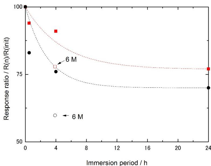
Figure 3. Response ratio to 1 mM glucose before and after immersion of the electrode in 3 M urea. The red squares represent cellulose-based GOD membranes. The black circles represent polyion complex membranes containing GOD. The open marks represent immersion in 6 M urea.
