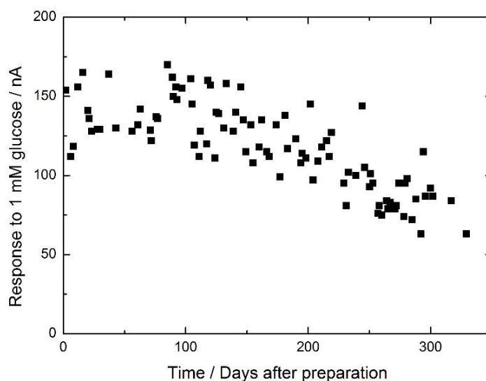
Figure 2. Long-term stability of the cellulose-based glucose oxidase (GOD) membrane. The daily response of the electrode to 1 mM glucose is shown.
