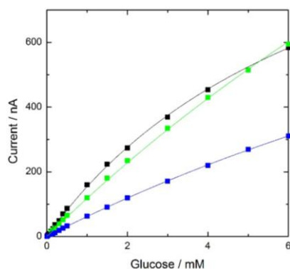
Figure 1. Calibration curves of glucose based on cellulose-based glucose oxidase membrane electrode. The black curve was obtained on the 2nd day after preparation. The green and the blue curves were obtained on 117th day and 329th day, respectively.
