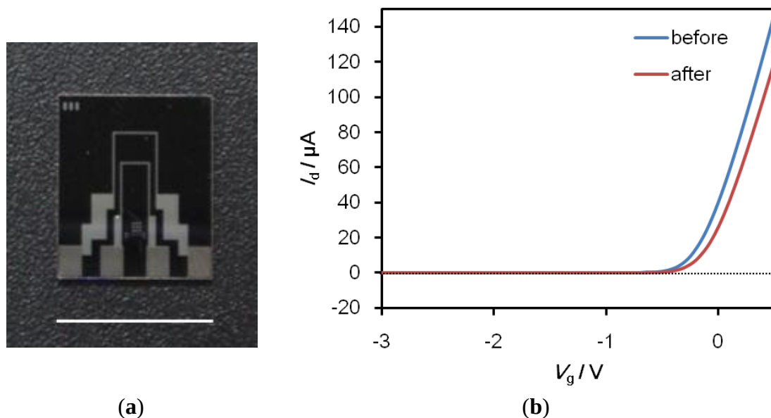
Figure 6. (a) Optical microscopic image of the FET device fabricated through the semiconductor processes. The bar indicates 10 mm; (b) Change in the V_g - I_d characteristics of FET device before and after the addition of the proteins.
