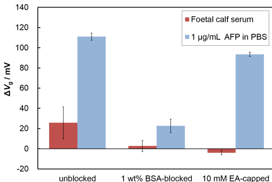
Figure 4. Comparison of sensor response to protein addition for antibody-immobilized FET (non-blocked, bovine serum albumin (BSA)-blocked, and ethanolamine-capped). The proteins were foetal calf serum for negative control and AFP (1 \mu\text{g/mL} ) for positive control.
