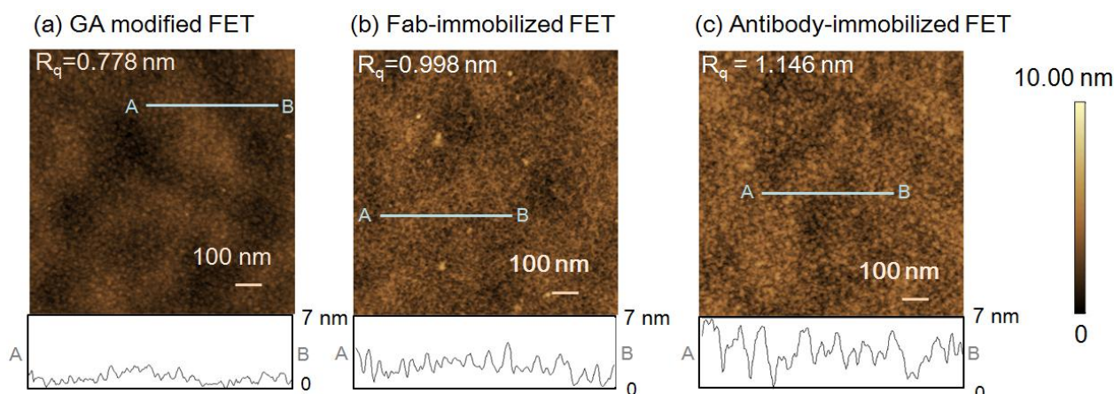
Figure 1. Atomic force microscope (AFM) images of the field-effect transistor (FET) gate surface obtained after (a) introduction of glutaraldehyde (GA); (b) immobilization of Fab; and (c) immobilization of whole antibody. Z range = 10 nm. Each image has a cross-sectional profile shown.
