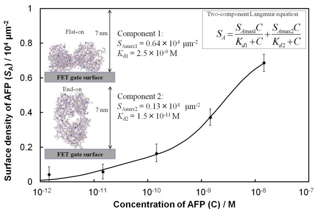
Figure 3. Surface density of AFP, calculated from the magnitude of \Delta V_g and the charge of AFP (see text), as a function of AFP concentration. Inset shows the schematic representation of the two different orientations of Fab on surfaces and the two-component Langmuir-type adsorption model equation.
