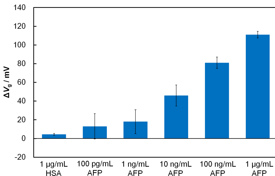
Figure 2. Relation between \alpha -fetoprotein (AFP) concentration and \Delta V_g magnitude for Fab-immobilized FET.
