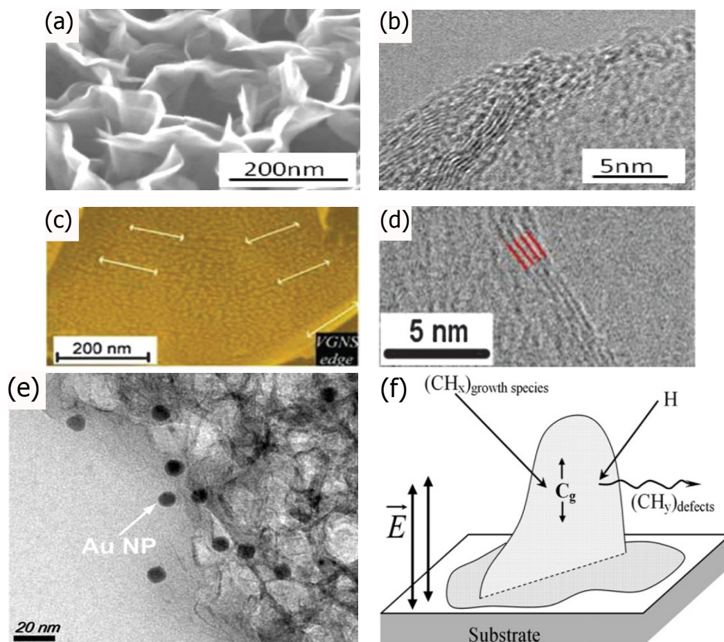
Figure 6. Structures, morphologies, and growth mechanism for plasma-enabled catalyst-free growth of few-layer CNWs. (a) High-resolution SEM of ultra-thin CNWs produced from natural honey; (b) high-resolution TEM image of the graphitic edges of CNWs. Reproduced from [201]; (c) CNWs with self-organised AuNP arrays; (d) high-resolution TEM image of 4-layer VGs. Reproduced from [202]; (e) AuNPs introduced into CNWs by electrodeposition. Reproduced from [198]; (f) growth model for CNWs. Reproduced from [215].
