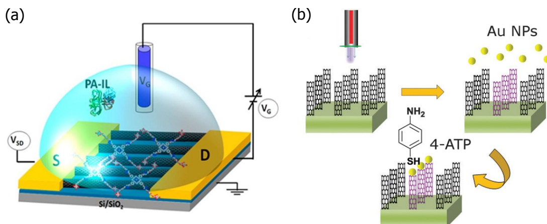
Figure 3. Carbon nanotubes (CNT)-based biosensors including FETs, vertically aligned CNT arrays for SERS, CNTs for Raman tags, and fluorometric CNT arrays. (a) Schematic of an electrolyte-gated CNT-FET, in which CNT walls were noncovalently functionalized with porphyrin-based glycoconjugates. Reproduced from [162]; (b) Outline of the vertically aligned CNTs functionalization with AuNDs with an atmospheric pressured plasma jet (APPJ). Reproduced from [163]; (c) Multi-color SWCNT Raman labels for multiplexed protein detection; (d) Demonstration of the G-mode Raman scattering spectra of ^{12}\text{C} (red) and ^{13}\text{C} (green) SWCNT Raman tags. Reproduced from [164]; (e) A SWCNT/chitosan suspension was spotted on glass and functionalized with Ni-NTA to bind His-tag-containing capture proteins; (f) Illustration of the fluorescence change ( \Delta I/I_0 ) following the immobilization of capture proteins and its subsequent binding with the analyte proteins on the SWCNT/chitosan array. Reproduced from [165].
