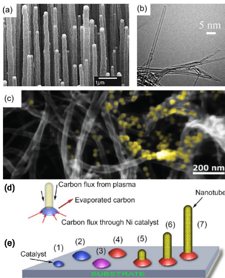
Figure 4. Plasma-enabled growth of vertically aligned carbon nanotubes (CNTs), including CNT structures, morphologies, AuNP modification and growth mechanism. (a) MWCNTs fabricated on nickel-coated glass by PECVD. Reproduced from [185]; (b) TEM of SWCNTs deposited on SiO 2 wafer/Si substrate via PECVD (<750 °C) with fast heating. Reproduced from [186]; (c) Vertically aligned CNTs treated by cold atmospheric-pressure micro-plasma jet (APMPJ) for the decoration of AuNDs. Reproduced from [163]; (d) Overview of CNT growth from CNP nucleation to termination; (e) The seven main stages of the formation of the carbon nanostructure pattern on the surface. Reproduced from [30].
