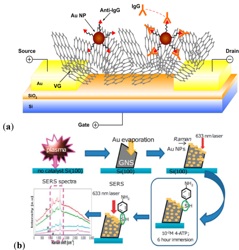
Figure 5. Carbon nanowalls (CNW)-based FET and plasmonic/SERS-active biosensing platforms. (a) A CNW substrate was decorated with AuNP-anti-IgG conjugates by electrodeposition, for the sensing of complementary IgGs. Reproduced from [198]; (b) CNWs synthesized on Si(100) substrate via a catalyst-free N_2 PECVD. The thermally evaporated AuNPs were self-assembled onto the CNWs as a SERS platform. Reproduced from [202].
