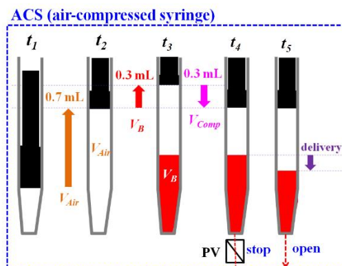
Figure A1. Fabrication and operation of the air-compressed syringe. (A) Two air-compressed syringes (ACSs) filled with blood sample ( Hct = 50\% ) and reference fluid (RBCs in 40% glycerin sol. [ Hct = 7\% ]). Each ACS was composed of a disposable syringe ( \sim 1\text{mL} ), a fixture, and a pinch valve. (B) Operation of ACS: piston movement at the lowest position forward at t = t_1 , air suction ( V_{\text{Air}} = 0.7 \text{ mL} ) by moving piston to 0.7 mL backward at t = t_2 , blood suction by moving piston to 0.3 mL backward ( V_B = 0.3 \text{ mL} ) at t = t_3 , air compression by moving piston to 0.3 mL forward ( V_{\text{comp}} = 0.3 \text{ mL} ) at t = t_4 , and blood delivery by removing pinch valve at t = t_5 . Similarly, the reference fluid was sucked into the syringe instead of blood. The remaining procedure was the same as blood delivery with the ACS. The blood sample and reference fluid were then delivered into the corresponding inlets with two ACSs. (C) Snapshots for showing RBC-free liquid in a tube under blood delivery using an ACS. Owing to the continuous erythrocyte sedimentation rate (ESR) inside the ACS, a red blood cell (RBC)-free liquid was observed in the microfluidic channel after a certain lapse of time.
