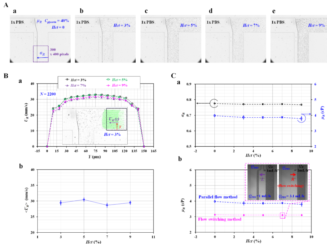
Figure 2. Contributions of RBCs added into the reference fluid to viscosity. 1x PBS was delivered to the blood channel at a constant flow rate of 1 mL/h with a syringe pump (SP). The hematocrit ( Hct ) of reference fluid was adjusted by adding normal RBCs into 40% glycerin solution ( Hct = 0, 3\%, 5\%, 7\% , and 9\% ). The reference fluid was delivered to the reference channel at a constant flow rate of 1 mL/h with an SP. (A) Microscopic images for obtaining interface ( \alpha_R ) in co-flowing channel with respect to Hct ((a) Hct = 0 , (b) Hct = 3\% , (c) Hct = 5\% , (d) Hct = 7\% , and (e) Hct = 9\% ). (B) Contributions of hematocrit in reference fluid to velocity fields ( U_R ). (a) Variation of velocity fields ( U_R ) across reference channel width with respect to Hct . The inset showed a microscopic image and a velocity profile of the reference fluid with Hct = 3\% . (b) Variations of \langle U_R \rangle averaged over a region of interest (ROI) with respect to Hct . (C) Effect of Hct in reference to fluid on viscosity ( \mu_R ). (a) Variations of \alpha_R and \mu_R with respect to Hct . (b) Comparison between the proposed method (i.e., the parallel-flow method with correction factor) and previous method (i.e., flow-switching method) with respect to Hct .
