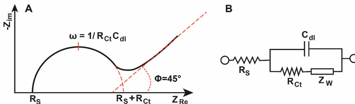
Figure 5. The Nyquist plot (A) and the corresponding Randles circuit (B).
