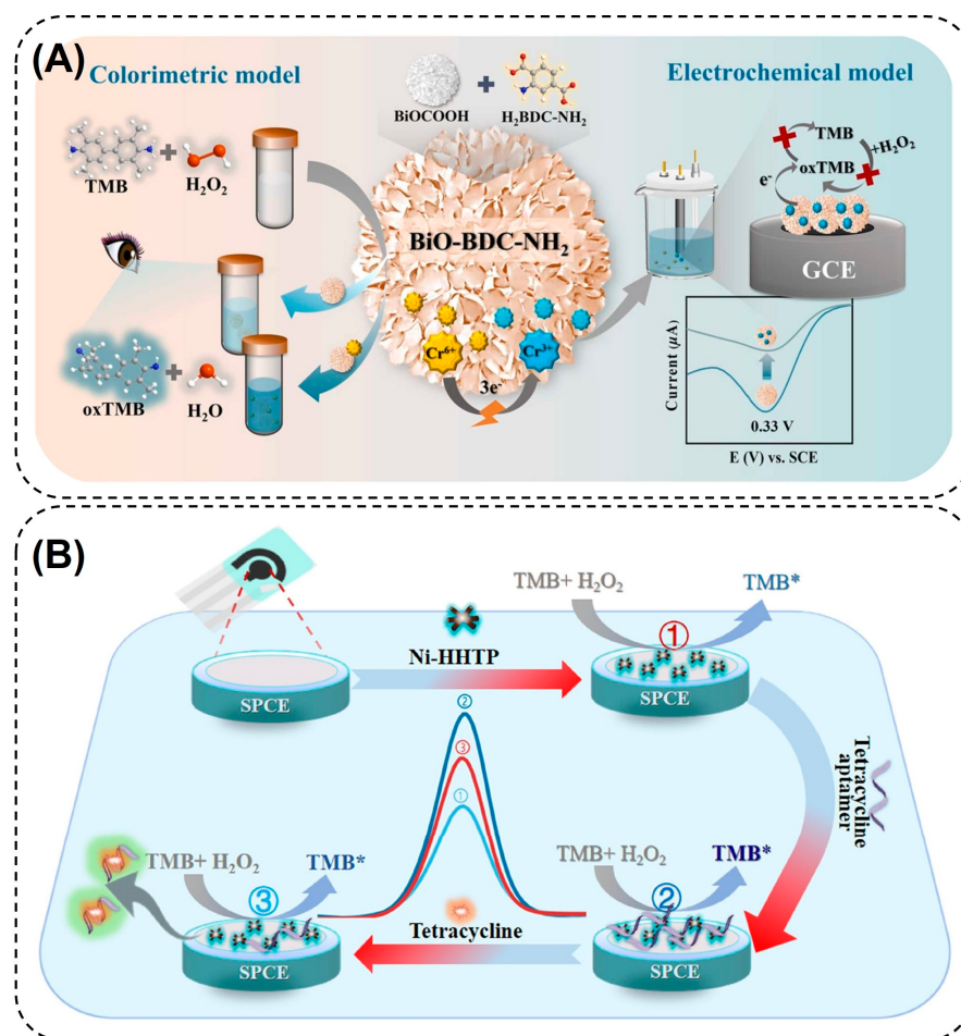
Figure 8. MOF-NZ-based electrochemical biosensor. Schematic illustration of the electrochemical (A) and colorimetric \text{Cr(VI)} ion detection by using POX-mimic \text{BiO-BDC-NH}_2 MOF. Reproduced with permission from [182] and (B) tetracycline residue detection by using POX-mimic \text{Ni-HHTP} MOF, ( \text{TMB}^* : oxidized TMB). Reproduced with permission from [186].
