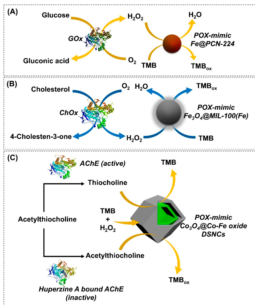
Figure 6. MOF-NZ-based colorimetric biosensors. Schematic illustration of (A) glucose and H_2O_2 detection by employing GOxFe@PCN224 MOFs. Adapted with permission from [120]; (B) cholesterol detection by employing ChOxFe_3O_4@MIL-100(Fe) MOFs. Adapted with permission from [61]; and (C) AChE activity detection in the absence and presence of huperzine A (AChE inhibitor) by utilizing Co_3O_4@Co-Fe oxide DSNC MOFs. Adapted with permission from [65].
