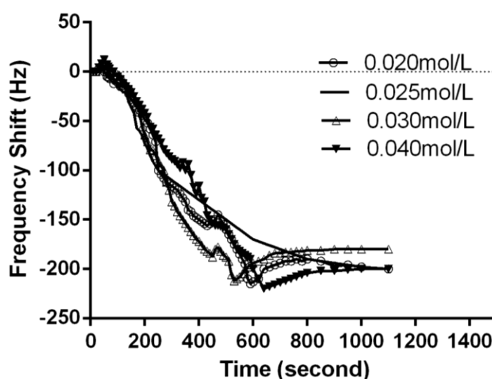
Figure 3. The effect of calcium chloride concentration on coagulation reaction.
