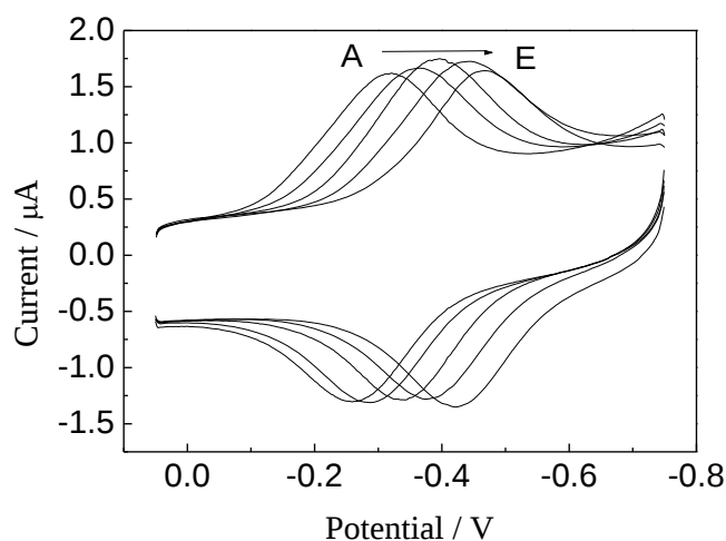
Figure 6. Cyclic voltammograms for Hb/GNPs-GR-SDS/BPG modified electrode at scan rate 0.1 \text{ V}^{-1} in buffer solutions at different pH values. pH value (from A to E): 5, 6, 7, 8 and 9.
