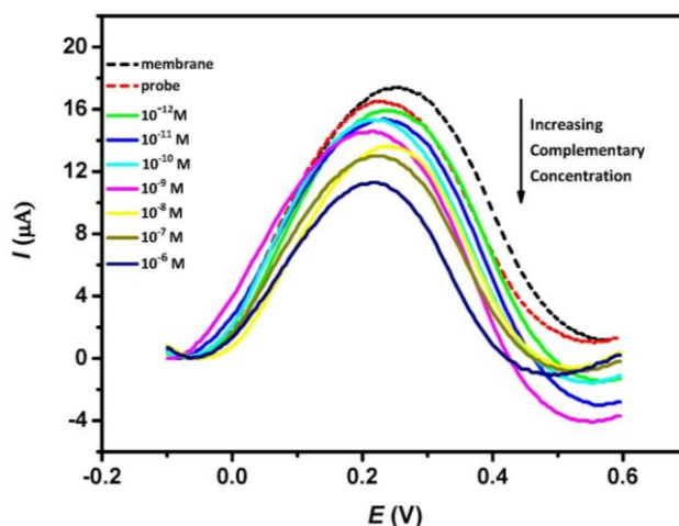
Figure 2. Differential pulse voltammetry current signal response of the integrated nanoporous membrane sensor toward increasing concentration of complementary DNA target from 10^{-12} to 10^{-6} M.
