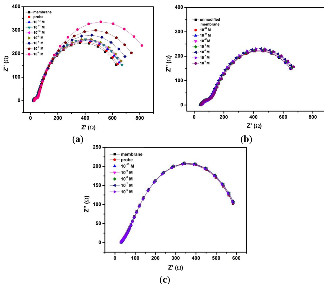
Figure 3. Nyquist plots of (a) integrated nanoporous membrane electrode grafted with DNA probe, (b) unmodified nanoporous membrane electrode in response toward increasing concentrations of target DNA ( 10^{-12} ~ 10^{-6} M), (c) 200 nm pore size membrane sensor grafted with DNA probe toward increasing concentration of DNA targets ( 10^{-10} ~ 10^{-6} M).
