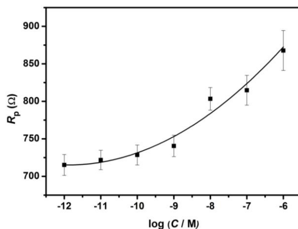
Figure 4. Calibration plot of pore resistance against the logarithm of complementary target DNA concentration.
