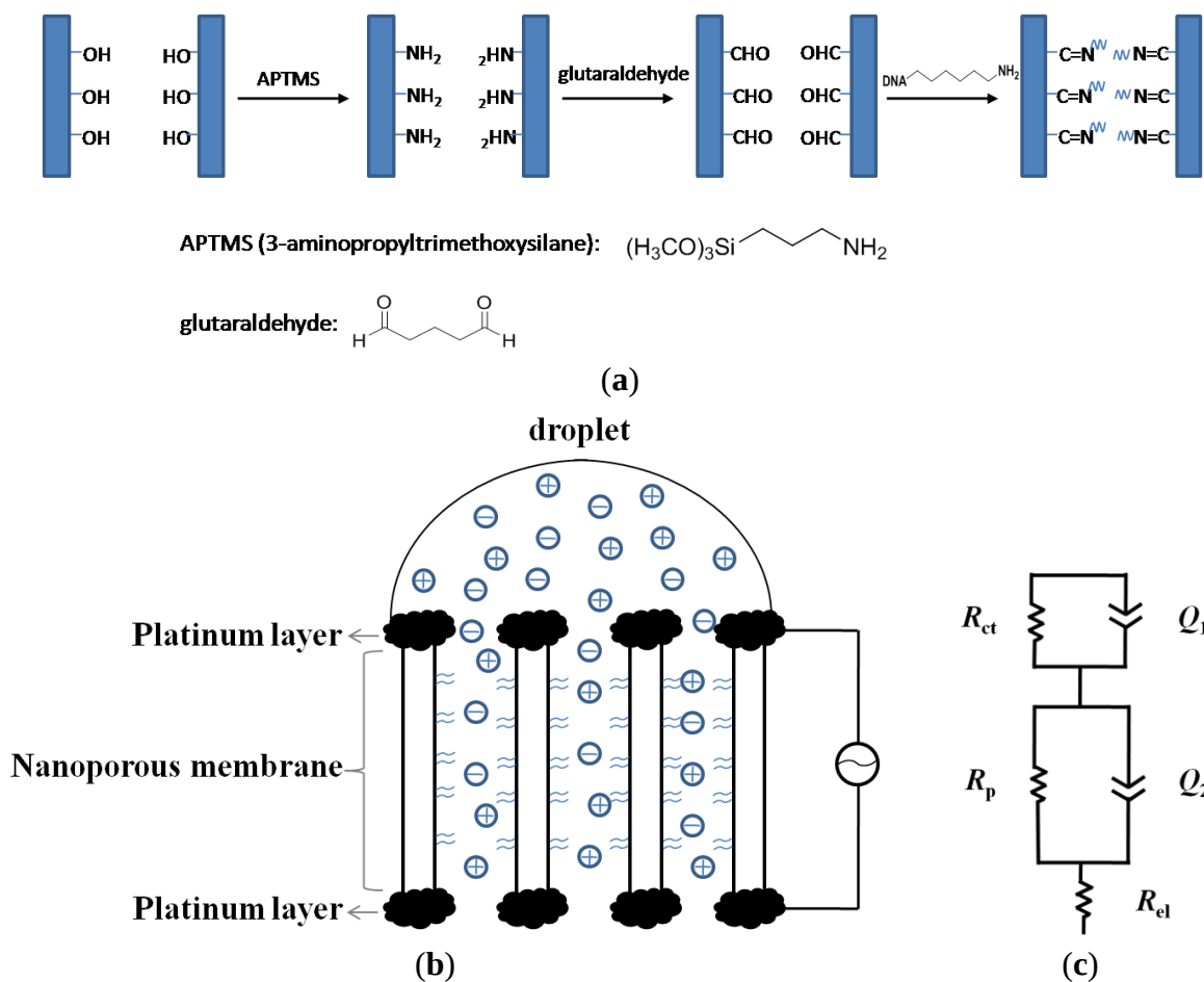
Figure 1. (a) Scheme of DNA immobilization procedure; (b) Schematics of nanoporous alumina membrane for impedimetric biosensing of DNA target; (c) The equivalent circuit model for fitting the impedimetric experimental data.
