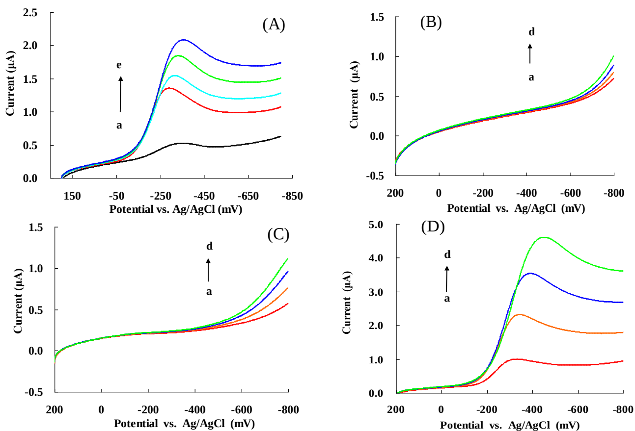
Figure 4. LSVs of (A) NF/Hb/FMWCNTs/Cys/AuNPs/GC electrode in the absence or presence of different concentrations of \text{H}_2\text{O}_2 (from curve a to curve e): 0, 0.1, 0.13, 0.16, 0.20 mM, respectively. LSVs of (B) Cys/AuNPs/GC; (C) NF/Cys/AuNPs/GC and (D) NF/Hb/Cys/AuNPs/GC electrodes, respectively in the presence of different concentrations of \text{H}_2\text{O}_2 (from a to curve d): 0.1, 0.3, 0.5 and 0.7 mM, respectively.
