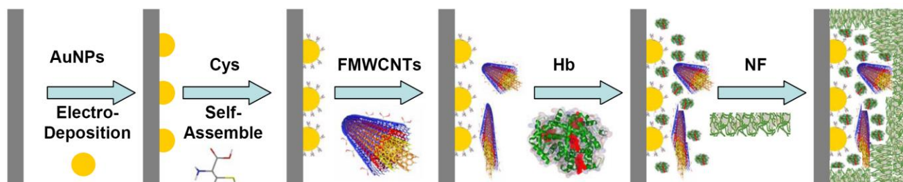
Figure 1. Preparation process of functional membrane modified glassy carbon (GC) electrode.
