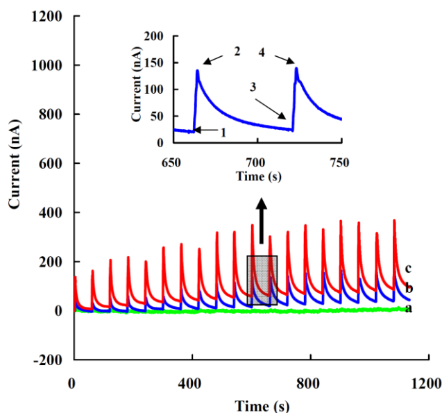
Figure 5. Amperometric response of the modified electrode to successive additions of 5 \mu\text{L} of 1 nM (a), 10 nM (b) or 20 nM (c) \text{H}_2\text{O}_2 in 5 mL of 0.05 M PBS, pH 7.0, at the applied potential of -0.35 V (vs. Ag/AgCl). Inset shows the typical current response for each addition process: (1) previous steady state current; (2) maximum response current; (3) steady state current; (4). next maximum response current.
