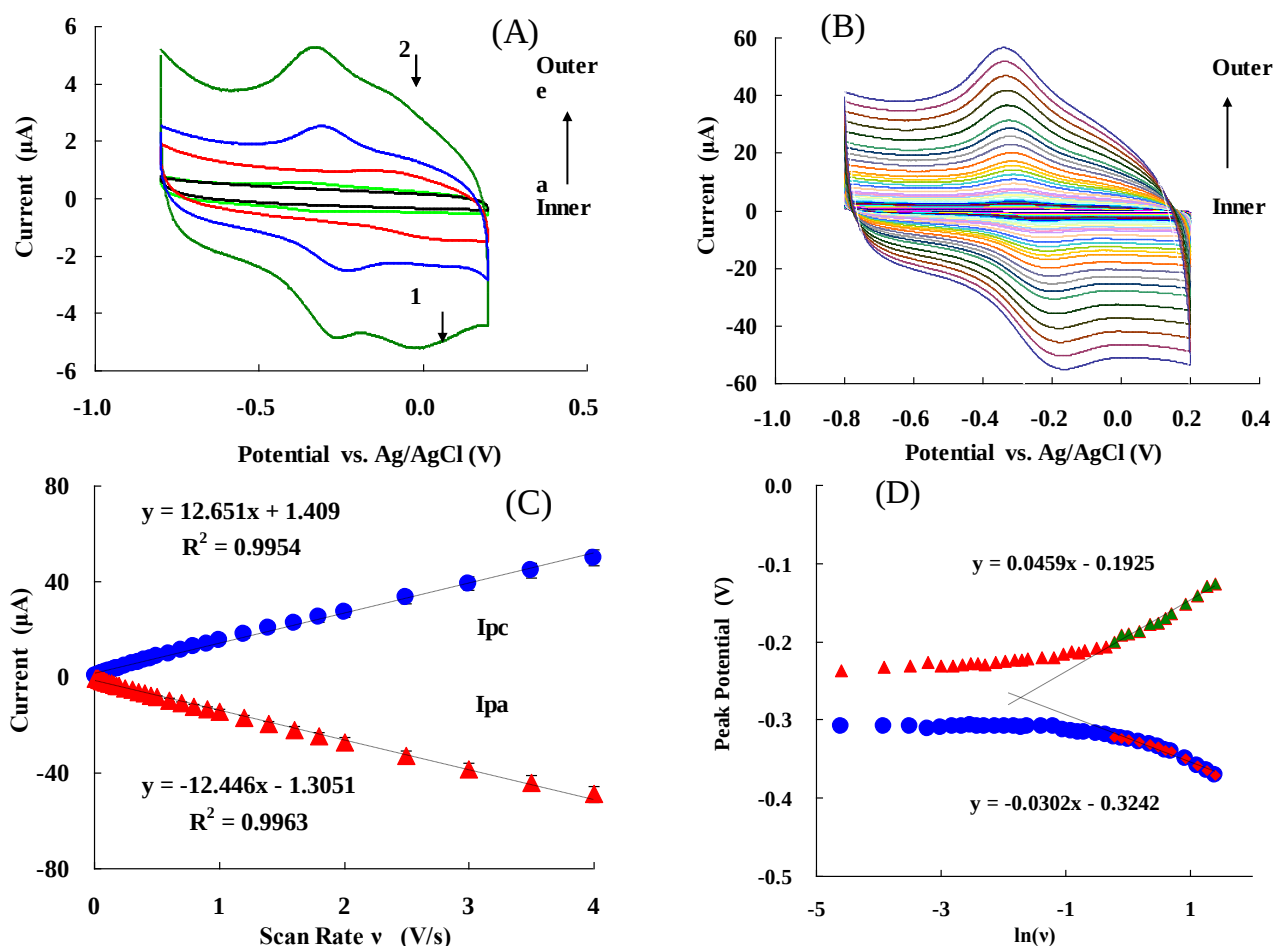
Figure 2. (A) CVs of different modified electrodes (from inner to outer): (a) Bare GC electrode; (b) NF/Hb/GC; (c) NF/FMW/CNTs/Cys/AuNPs/GC; (d) NF/Hb/FMW/CNTs/GC; (e) NF/Hb/FMW/CNTs/Cys/AuNPs/GC. The experiments were carried out in 0.05 M PBS (pH 7.0) at a scan rate of 0.05 V/s. (B) CVs of NF/Hb/FMW/CNTs/Cys/AuNPs/GC electrode in 0.05 M PBS (pH 7.0) at various scan rates (from inner to outer): 0.02, 0.04, 0.06, 0.08, 0.1, 0.12, 0.14, 0.16, 0.18... 4 V/s, respectively; (C) Plot of peak current I_p vs. scan rate v ; (D) Plot of peak potential E_p vs. \ln(v) .
