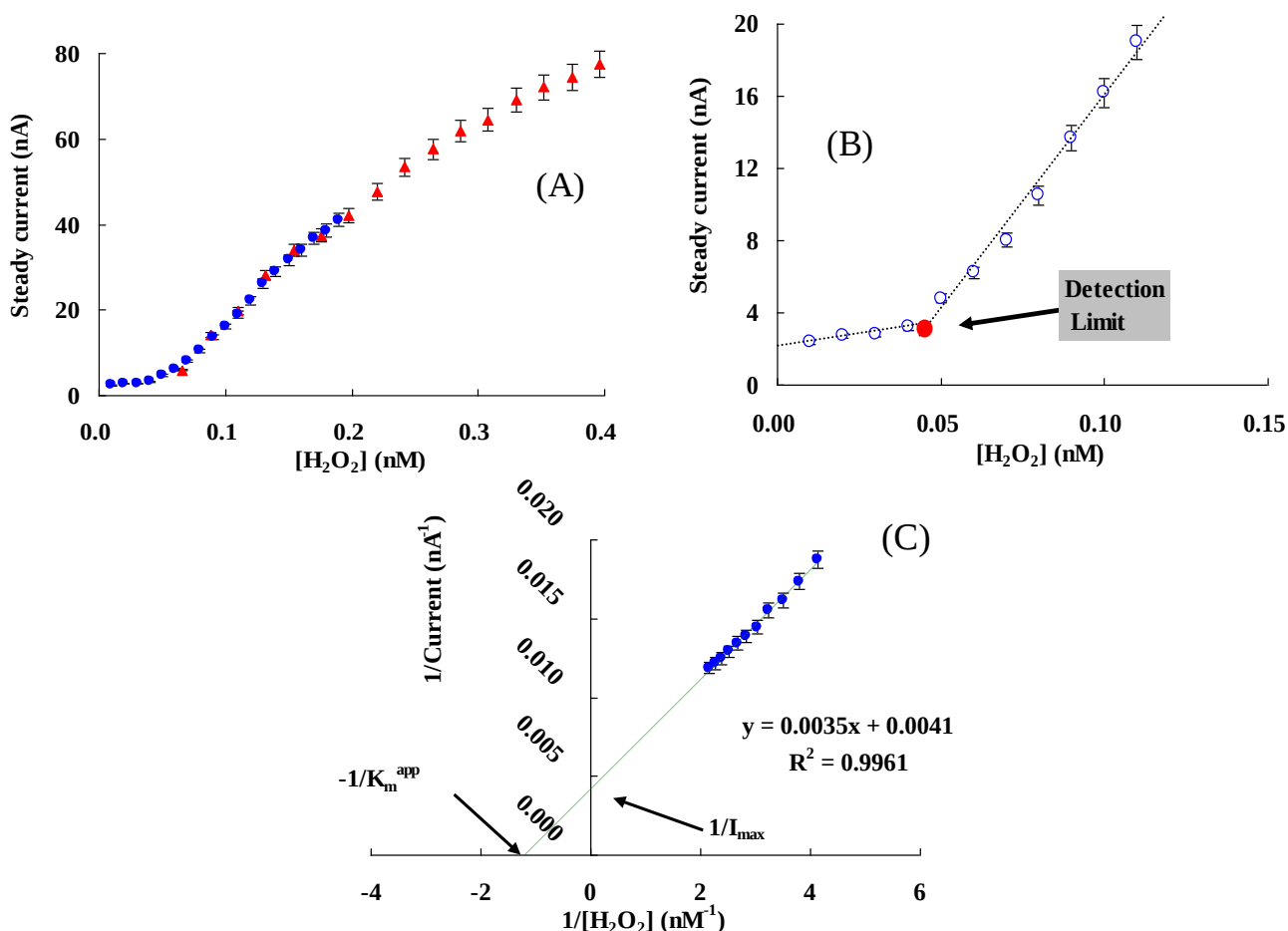
Figure 6. (A) The typical steady current vs. [\text{H}_2\text{O}_2] in the process of successive additions of 5 \mu\text{L} of 10 nM (●) and 20 nM (▲) \text{H}_2\text{O}_2 in 5 mL of 50 mM PBS (pH 7.0) at the applied potential of -0.35 V (vs. Ag/AgCl). (B) The determination of the \text{H}_2\text{O}_2 detection limit for NF/Hb/FMWCNTs/Cys/AuNPs/GC electrode. The detection limit was determined from the cross point of the lines fitted to the linear segments of the steady current I_s vs. [\text{H}_2\text{O}_2] in the process of successive additions of 5 \mu\text{L} of 10 nM \text{H}_2\text{O}_2 in 5 mL of 50 mM PBS (pH 7.0). (C) Lineweaver-Burk plot for K_m^{\text{app}} determination.
