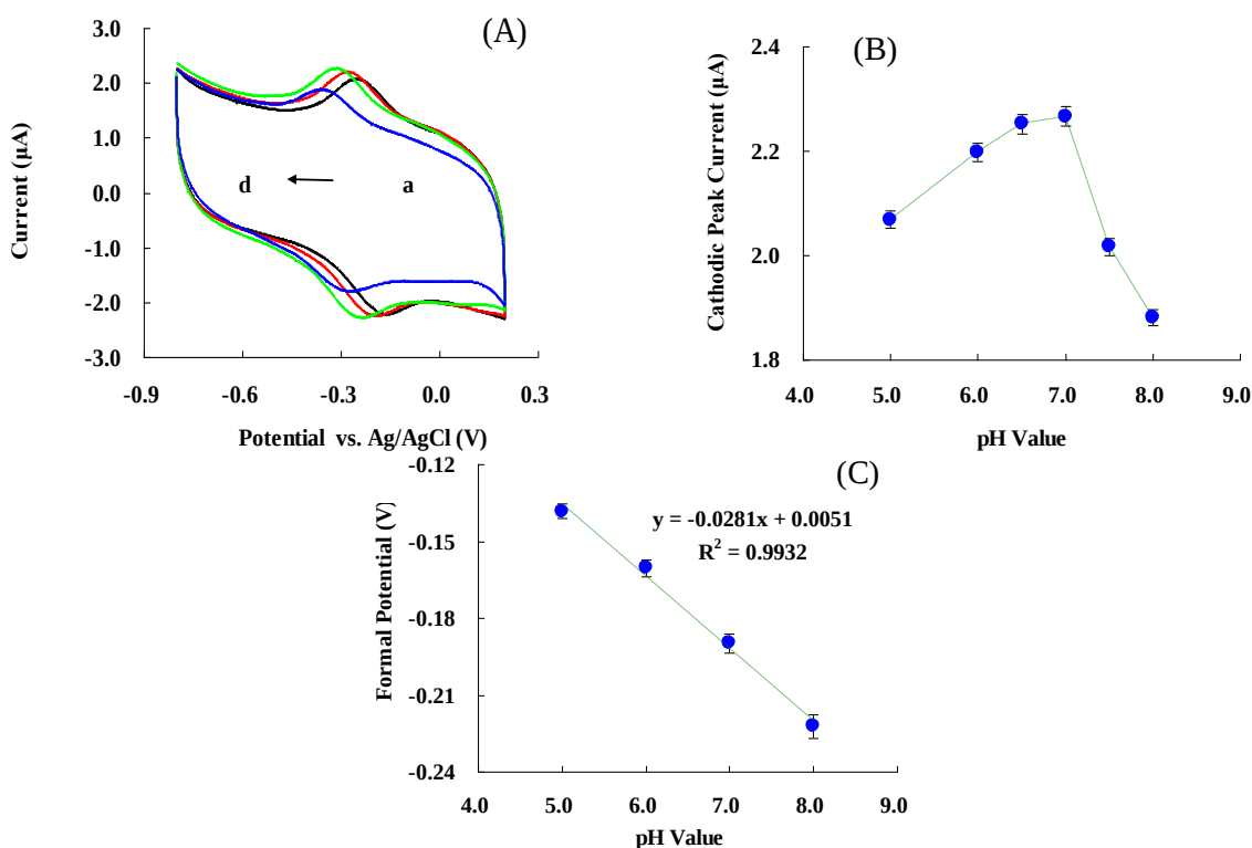
Figure 3. (A) CVs of NF/Hb/ FMWCNTs/Cys/AuNPs/GC electrode in 0.05 M PBS at different pH values: (a) 5.0, (b) 6.0, (c) 7.0, and (d) 8.0, respectively; (B) plot of I_{pc} vs. pH value; (C) Plot of E^\circ vs. pH value.
