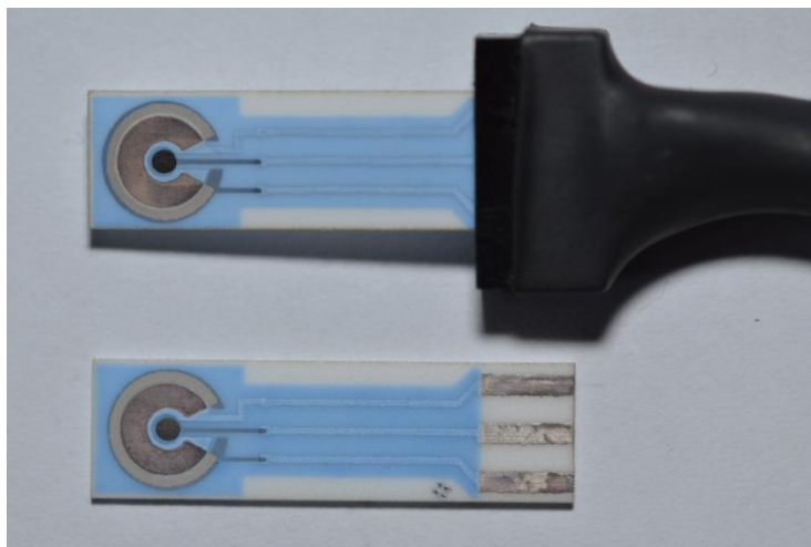
Figure 1. Screen printed sensors used in the experiments. In the upper part, sensor in a plastic holder is depicted. In the bottom part, a naked sensor is shown. Electrodes are on the left side of the picture, output contacts on the right.
