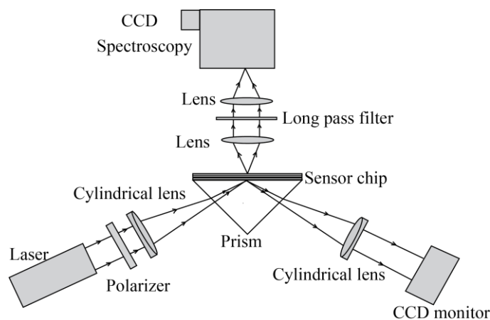
Figure 2. Schematic of the hyperspectral fluorescence detections based on a symmetrical CPWR structure.
