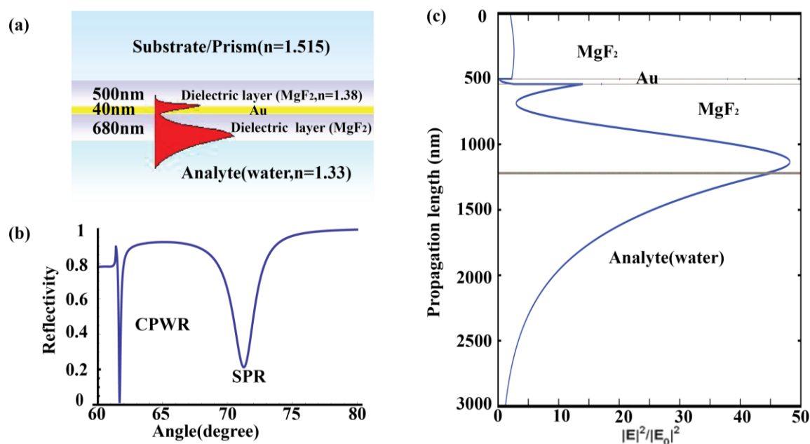
Figure 1. (a) 1D implementation of a symmetrical optical waveguide structure based on Kretschmann configuration for CPWR excitation. Theoretically calculated angular reflectivity curves (b) and electric field distributions (c) for the architecture given in (a) at the excitation wavelength of 632.8 nm, n(\text{Au}) = 0.3123 + 3.146i . Propagation length in this figure refers to the electric field decay distance away from the sensor surface into the analyte.
