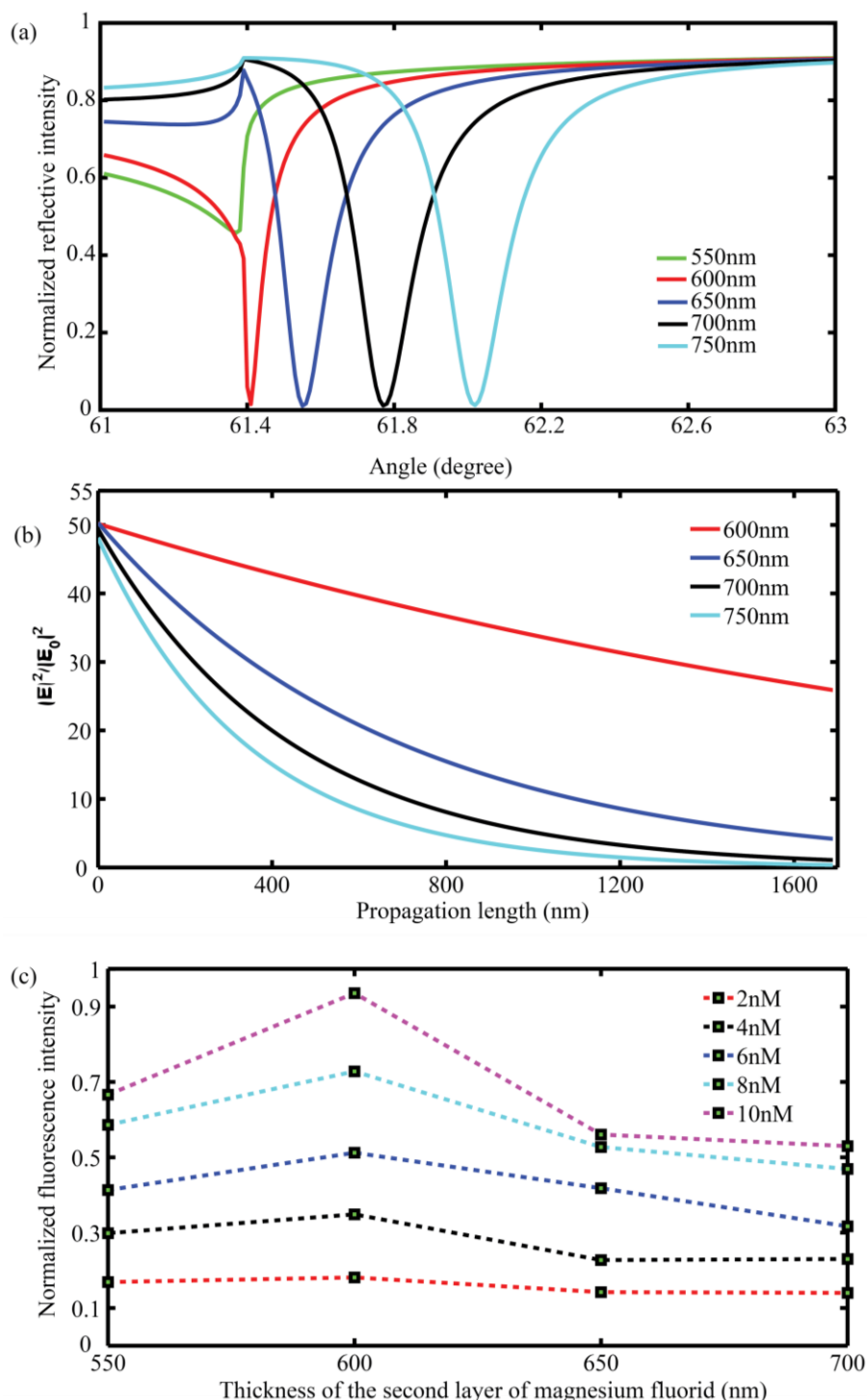
Figure 4. Resonance curves (a) and electric field distribution (b) beyond the sensor films directly into sensed medium simulated with various thicknesses of second layer of magnesium fluoride 600 nm (red), 650 nm (blue), 700 nm (black), 750 nm (cyanine) generated by symmetrical CPWR. Thicknesses of the first layer of magnesium fluoride and Au metal film are 500 nm and 40 nm, respectively. Wavelength of the incident light is 632.8 nm, n(\text{BK}_7) = 1.515 , n(\text{MgF}_2) = 1.38 , n(\text{Au}) = 0.3123 + 3.146i ; (c) Fluorescence intensities against to different concentrations responding to sensor films with different thicknesses of second \text{MgF}_2 layer ranging from 550 nm to 700 nm.
