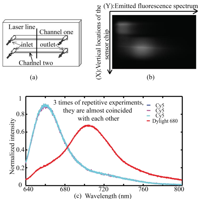
Figure 3. Demonstration of the data processing. (a) Structure of the two flow channels and the focused laser line; (b) An image captured by CCD, corresponding to the irradiated line region; (c) Fluorescence spectra correspond to channel one and channel two separately. Thicknesses for the three successive layers of \text{MgF}_2 -Au- \text{MgF}_2 are 500 nm, 40 nm, 600 nm individually.
