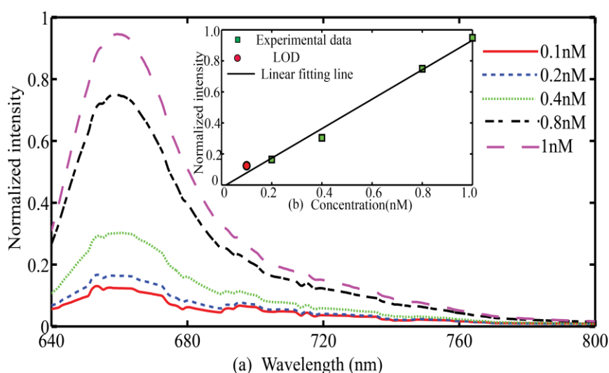
Figure 5. (a) Fluorescence spectra for each concentration; (b) Plot of normalized fluorescence intensities against solution concentrations.
