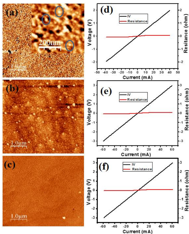
Figure 1. (a) AFM image of the InN QDs grown on an InGaN layer. Inset: AFM image with enlarged magnification. Some InN QDs are encircled for clarification; (b) AFM image of the InN thin film grown on an InGaN layer; (c) AFM image of the bare InGaN layer; (d–f) I–V curves measured with two Al ohmic contacts deposited on the InN QDs, InN thin film, and InGaN layer, respectively.
