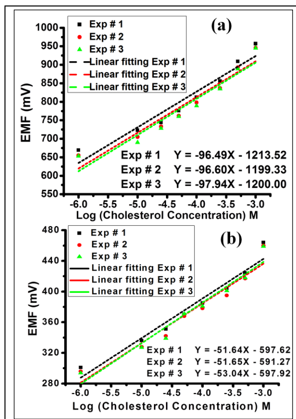
Figure 3. (a,b) EMF as a function of the logarithmic cholesterol concentration of the InN QDs and InN thin film based biosensors, respectively. Exp # 1–3 denote three different experiments.
