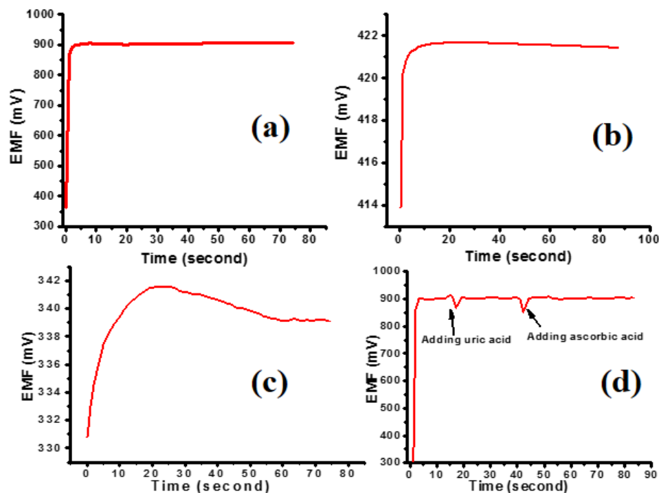
Figure 4. (a) EMF as a function of time of the InN QDs based biosensor for 500 \mu\text{M} cholesterol concentration; (b) EMF as a function of time of the InN thin film based biosensor for 500 \mu\text{M} cholesterol concentration; (c) EMF as a function of time of the InGaN layer based biosensor for 500 \mu\text{M} cholesterol concentration; (d) EMF as a function of time when adding 50 \mu\text{M} uric acid (UA) and ascorbic acid (AA) to the 500 \mu\text{M} cholesterol solution.
