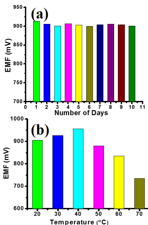
Figure 5. (a) Repeated experiments for ten consecutive days for 500 \mu\text{M} cholesterol concentration using same InN QDs-based biosensor; (b) EMF as a function of temperature of the InN QDs-based biosensor for 500 \mu\text{M} cholesterol concentration.
