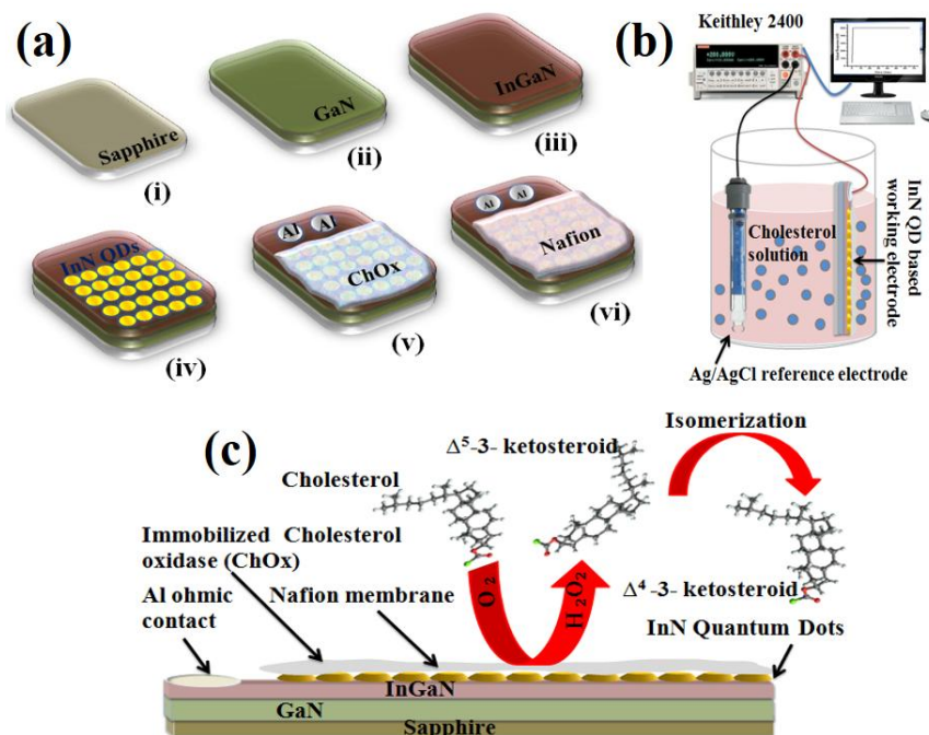
Figure 2. (a) Schematic diagram of the fabrication process of the biosensor; (b) Schematic illustration of the sensing setup using the working electrode comprised of the InN QDs coated with ChOx and a Ag/AgCl reference electrode; (c) Schematic illustration of the working electrode comprised of the InN QDs coated with ChOx along with the possible electrochemical reaction near the electrode.
