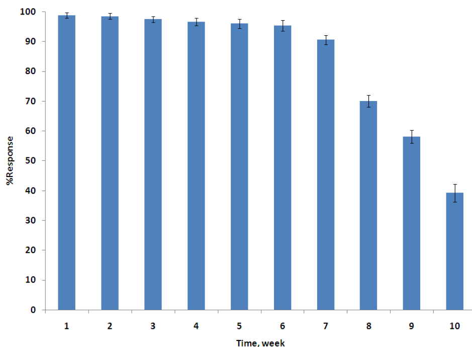
Figure 6. Stability of the AOX/PANI biosensor response (average of triplicate measurements) toward ethanol (1%) at pH buffer 7.0. within 1–10 weeks of storage (4 °C).
