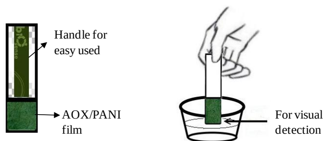
Figure 1. AOX/PANI film based biosensor design as a dip stick test (a) and simple use of sensor by dipped into sample solution (b).
