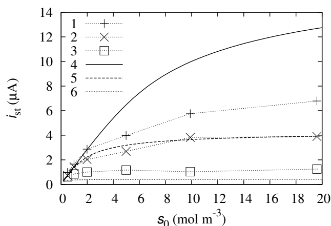
Figure 2. Experimental (1, 2, 3) and computational (4, 5, 6) calibration curves at different concentrations of the mediator ( m_0 ): 0.2 mol/m 3 (1, 4), 0.05 mol/m 3 (2, 5), 0.005 mol/m 3 (3, 6).
