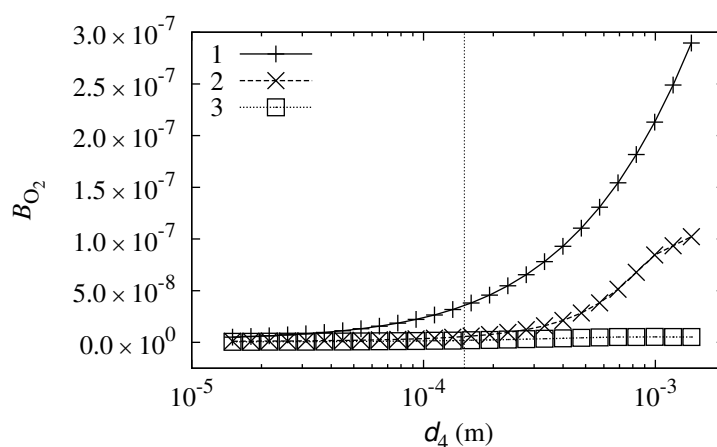
Figure 7. The biosensor response sensitivity, B_{O_2} , to oxygen dependence on the thickness, d_4 , of the diffusion layer at different values of the substrate concentration, s_0 : 0.498 \text{ mol/m}^3 (1), 4.98 \text{ mol/m}^3 (2) and 49.8 \text{ mol/m}^3 (3). The vertical line marks the estimated diffusion layer thickness during the physical experiment.
