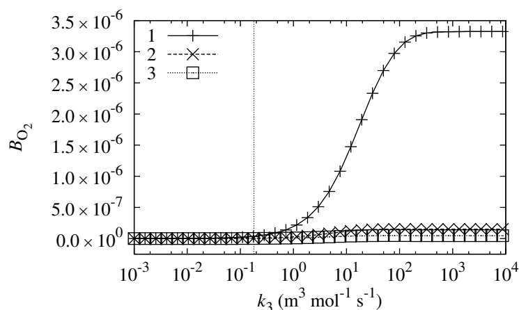
Figure 5. The biosensor response sensitivity, B_{O_2} , to oxygen dependence on reaction rate constant of Reaction (7), k_3 , at different values of substrate concentration s_0 : 0.498 mol/m 3 (1), 4.98 mol/m 3 (2) and 49.8 mol/m 3 (3). The vertical line marks the reaction rate constant, k_3 , corresponding to N-methylphenazonium methyl sulfate (PMS).
