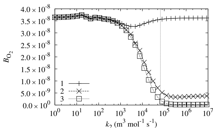
Figure 6. The biosensor response sensitivity, B_{O_2} , to oxygen dependence on reaction rate constant of Reaction (6), k_2 , at different values of substrate concentration s_0 : 0.498 mol/m 3 (1), 4.98 mol/m 3 (2) and 49.8 mol/m 3 (3). The vertical line marks the reaction rate constant, k_2 , corresponding to PMS.
