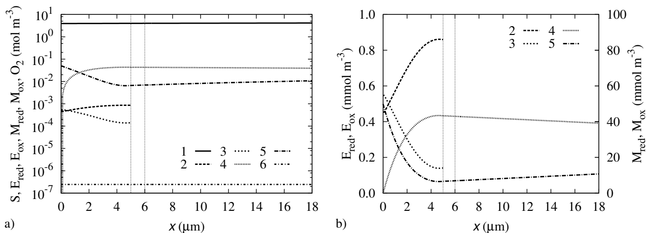
Figure 4. The concentration profiles of S (1), E_{\text{red}} (2), E_{\text{ox}} (3), M_{\text{red}} (4), M_{\text{ox}} (5) and O_2 (6) at the steady state. Vertical axes correspond to the concentration of species, horizontal axes correspond to the distance from an electrode surface. The vertical lines mark the boundaries of the biosensor layers. Concentrations in graph (a) are provided in logarithmic scale. In graph (b) concentrations of four species are depicted on a linear scale.
