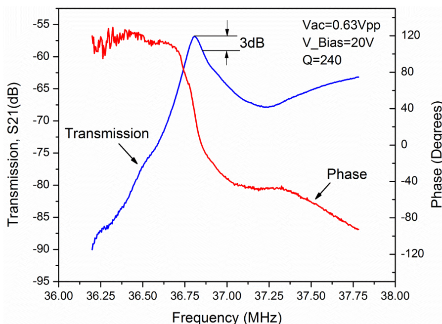
Figure 4. Measured S21 transmission of 36.8 MHz square resonator under DI water droplet (top surface contacted with water).
