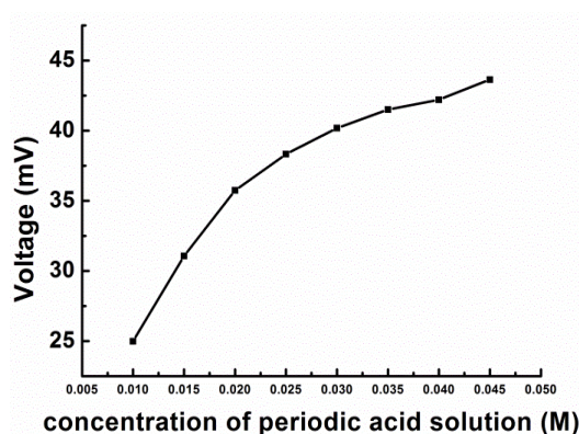
Figure 3. Effect of concentration of the periodic acid solution (pH 7) on the response of the FIA biosensor. A 350 \mu L sample of a 93.75 mg/L glucose solution was tested at a flow rate of 1.0 mL/min.
