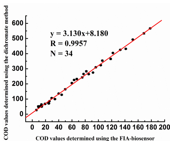
Figure 9. Graph showing the correlation between the COD values obtained using the FIA biosensor and those obtained using the dichromate method.
