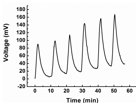
Figure 8. An actual sensor signal record for three determinations of 200 and 300 mg/L COD values.
