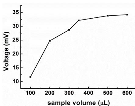
Figure 2. Effect of sample volume of a 93.75 mg/L glucose solution on the response of the FIA biosensor at a flow rate of 1.0 mL/min.
