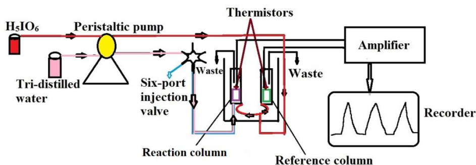
Figure 1. Schematic of the FIA biosensor.
