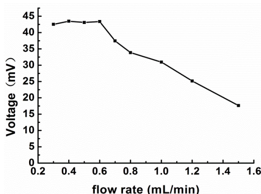
Figure 4. Effect of flow rate on the response of the FIA biosensor. A 350 \mu L sample of a 93.75 mg/L glucose solution was tested using a 0.03 M \text{H}_5\text{IO}_6 solution (pH 7).
