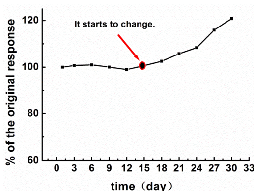
Figure 6. Stability of the response of the FIA biosensor with respect to a COD of 100 mg/L, as determined over 30 days.
