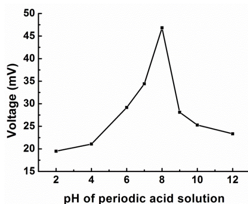
Figure 5. Effect of pH of \text{H}_5\text{IO}_6 on the response of the FIA biosensor. A 350 \mu\text{L} sample of a 93.75 mg/L glucose solution was tested using a 0.03 M \text{H}_5\text{IO}_6 solution at a flow rate of 0.6 mL/min.
