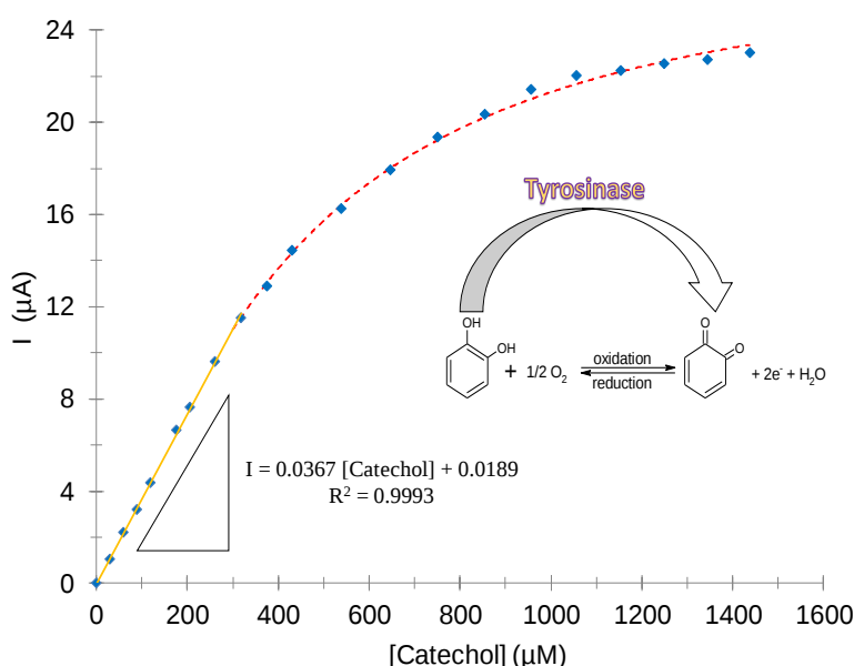
Figure 3. Enzymatic kinetics for catechol using mushroom tyrosinase in solution, in 0.1 M acetates' buffer at \text{pH } 4.50 \pm 0.01 and at (30.0 \pm 0.5)^\circ\text{C} . Following the measured current at -300 \text{ mV} imposed potential as a function of the catechol's concentration. The dots are experimental data and the line is the fitting of the Hill's model of Equation (1), the best fit parameters were K_m = (0.40 \pm 0.01) \text{ mM} , I_{\max} = (27.5 \pm 0.4) \mu\text{A} and h = 1.35 \pm 0.03 . The inset shows the reaction scheme of catechol and benzoquinone catalyzed by tyrosinase. The linear fit of the trace and its corresponding equation are also shown in the figure.
