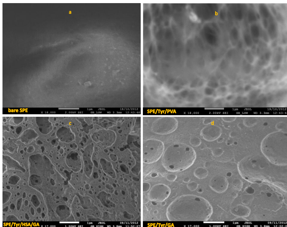
Figure 6. Results of the SEM morphology analysis of the bare SPE (a) and tyrosinase immobilized through: (b) entrapment, SPE/Tyr/PVA, (c) pure cross-linking with HSA, SPE/Tyr/HAS/GA and (d) cross-linking at (40.0 \pm 0.5)^\circ\text{C} , SPE/Tyr/GA.
