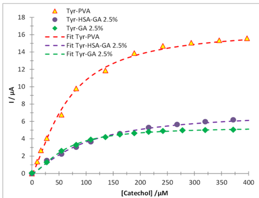
Figure 4. Comparison of the enzymatic kinetics for catechol (dots) recorded using the different tyrosinase biosensors: (▲) SPE/Tyr/PVA (●) SPE/Tyr/HSA/GA and (◆) SPE/Tyr/GA in acetates' buffer 0.1M at \text{pH } 4.50 \pm 0.01 a (30.0 \pm 0.5)^\circ\text{C} . Following the measured current, at -300\text{ mV} imposed potential, as a function of catechol's concentration. The lines correspond to the fitting of the Hill's model of Equation (1), the best fit values for K_m' , I_{\max} and h are shown in Table 1.
