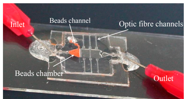
(b) Photonic microbeads sensor
