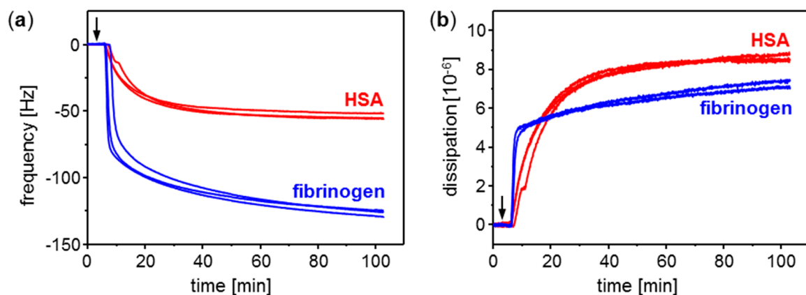
Figure 7. Conditioning film monitoring with QCM sensors coated with parylene C: Adsorption of plasma proteins HSA (red curves) and fibrinogen (blue curves). Samples contained 250 \mu\text{g/mL} protein in PBS. The PBS carrier stream was switched to sample solution 3 min after start of the measurement (see arrow). (a) Frequency; (b) Dissipation.
