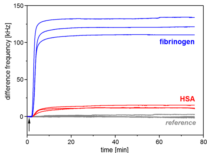
Figure 6. Conditioning film monitoring with SAW resonators coated with parylene C: Adsorption of plasma proteins HSA (red curves) and fibrinogen (blue curves). Samples contained 250 \mu\text{g/mL} protein in PBS and were injected into a PBS carrier stream. Injection started 1 min after start of the measurement (see arrow). Gray curves represent the signals obtained with the reference resonators, which were rinsed with carrier medium PBS throughout the complete measurement.
