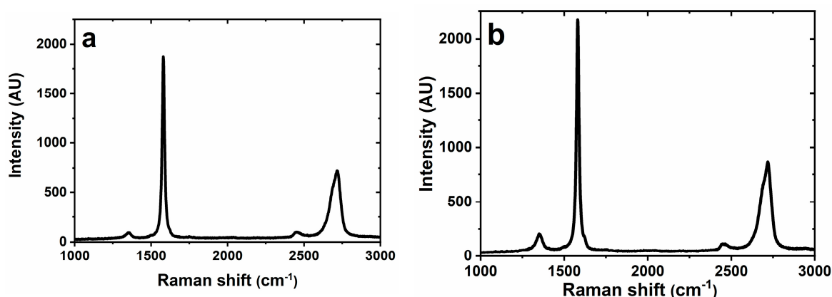
Figure 4. Raman spectra obtained for (a) plain graphene SPE and for (b) activated graphene SPE
