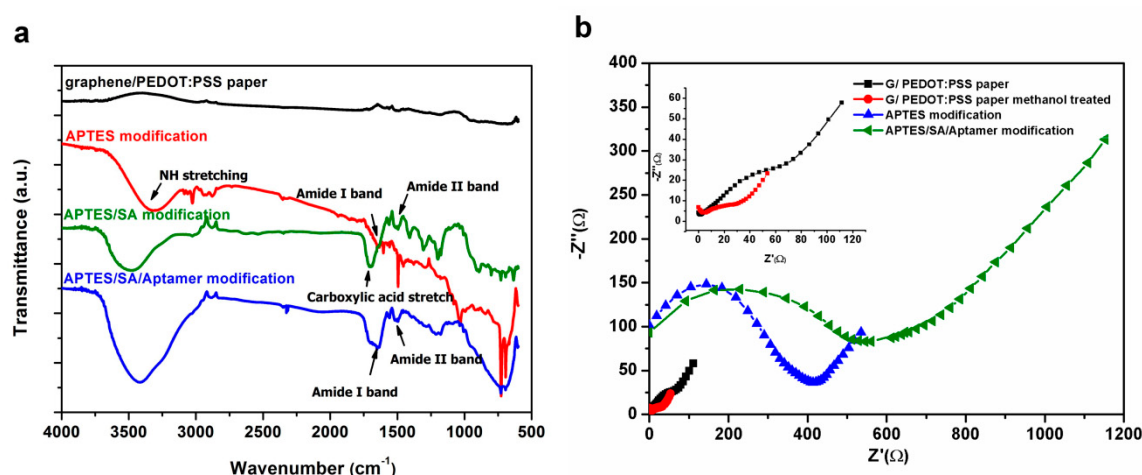
Figure 3. (a) The Fourier transform infrared (FTIR) spectra of a graphene/PEDOT:PSS paper electrode and (3-Aminopropyl)triethoxysilane (APTES) modified, APTES/SA modified and APTES/SA/Aptamer modified graphene/PEDOT:PSS paper electrode and (b) The electrochemical impedance spectroscopy (EIS) signal of graphene/PEDOT:PSS paper electrode in different surface functionalization steps.
