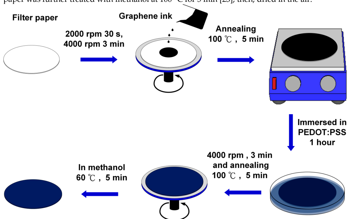
Scheme 1. Fabrication and modification process of the electrochemical paper-based working electrode: (1) paper cleaning; (2) graphene ink spin coating and annealing; (3) poly (3,4-ethylenedioxythiophene):poly(styrenesulfonate) (PEDOT:PSS) dip coating; (4) PEDOT:PSS spin coating and annealing; and (5) methanol treatment on the paper electrode.
