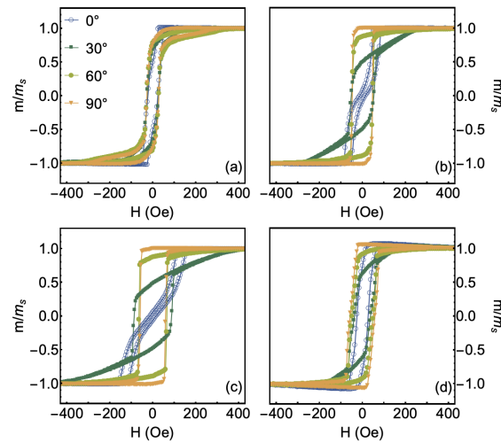
Figure 3. Normalized magnetization curves for the Co 2 FeAl/W bilayers grown onto GaAs (100) substrate, in which the CFA layer was deposited at the temperatures of (a) 300 K, (b) 573 K, (c) 673 K, and (d) 773 K. Here we present just the curves measured for \varphi = 0^\circ, 30^\circ, 60^\circ and 90^\circ . All the samples of the set present uniaxial magnetic anisotropy combined with cubic magnetic anisotropy, although these features are more evident for the ones produced at the temperatures of 573 K and 673 K.
