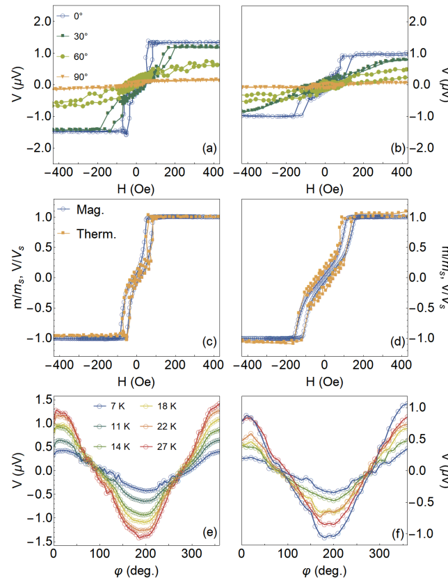
Figure 5. Experimental thermoelectric effect results. Thermoelectric voltage as a function of the magnetic field, at selected \phi values and setting \Delta T = 27 K, for the (a) CFA/W bilayers in which the CFA layer was grown at (a) 573 K and (b) 673 K. (c,d) Comparison of the shape of normalized magnetization and thermoelectric voltage curves acquired at \phi = 0^\circ , with \Delta T = 27 K, for these samples. (e,f) Angular dependence of the thermoelectric voltage at H = +500 Oe for distinct \Delta T values for the very same samples.
