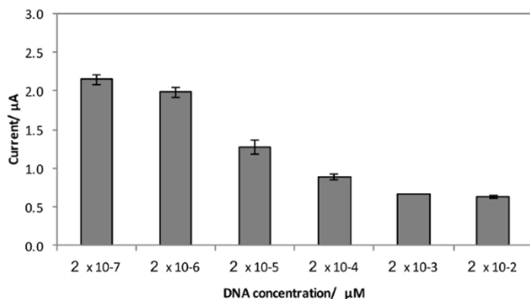
Figure 14: Histogram of the MB reduction peak current using different DNA concentration in 0.1 mol L -1 PBS (pH 7) at a scan rate of 0.1 V s -1 after 30 min incubation in 20 μM MB using differential pulse voltammetry measurement. Reprinted with permission from ref. [22]. Copyright (2016) Elsevier. Please click here to view a larger version of this figure.
