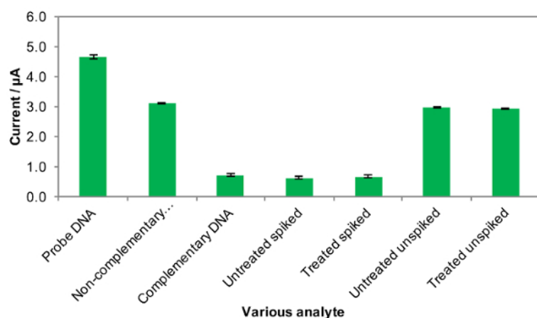
Figure 20: Histogram of the MB reduction peak current for detection of V. parahaemolyticus in fresh cockle samples using the DNA biosensor in 0.1 mol L -1 PBS (pH 7) at a scan rate of 0.1 V s -1 after 30 min incubation in 20 μM MB using differential pulse voltammetry measurement. Reprinted with permission from ref. [23]. Copyright (2017) Springer. Please click here to view a larger version of this figure.
