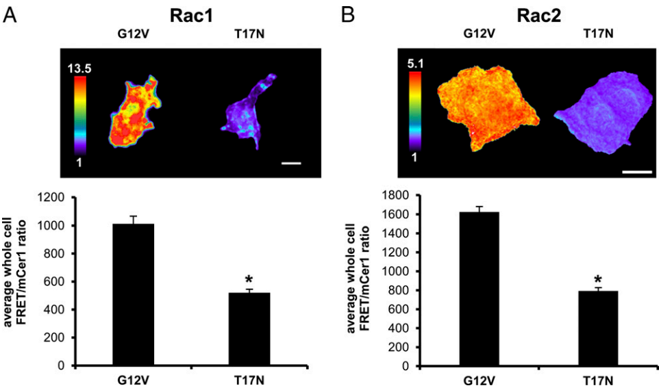
FIGURE 3. Validation of Rac1 and Rac2 biosensors in macrophages. (A) Ratiometric images of transiently overexpressed constitutively active (G12V) or dominant negative (T17N) Rac1 and (B) Rac2 biosensor (with mcp229Ven) in RAW/LR5 cells. Scale bar, 10 \mu m. Bar graphs are quantitation of whole cell levels of Rac activity. n = at least 15 cells per condition, mean \pm SEM. ^*p < 0.00001 .
