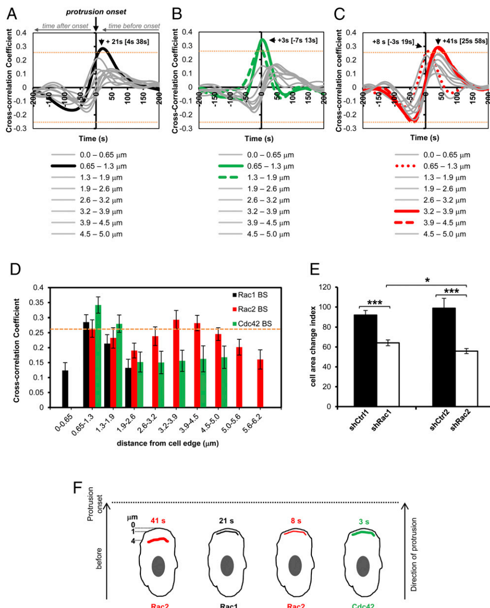
FIGURE 9. Morphodynamic analysis of Rac1, Rac2, and Cdc42 activation dynamics during random protrusions of macrophages. Temporal cross-correlation of GTPase activation relative to edge velocity, arrows showing peak activation times for (A) Rac1, (B) Cdc42, and (C) Rac2. Data from n = 733 windows from 25 cells for Rac1, n = 520 windows from 19 cells for Cdc42, and n = 778 windows from 29 cells for Rac2. Orange dashed line indicates that cross-correlations above 0.2552 or below -0.2552 are significant with p < 0.05 . Gray lines indicate nonsignificant correlations. See text for additional statistical values for morphodynamic analysis. (D) Spatial dependence of temporal cross-correlation of GTPase activation as a function of distance from the edge of the protrusion (data extracted from panels A–C). (E) Cell area change index for shRac1 and shRac2 macrophages and their respective controls, shCtrl1 and shCtrl2. Data are mean \pm SEM. (F) Model of Rho GTPase activation dynamics in random protrusions of macrophages showing that Rac2 is activated first in a 3.2–4.5- \mu\text{m} region 41 s before protrusion onset, followed by a second pool of Rac2 activation right behind the leading edge, in parallel with Rac1 and Cdc42, at indicated times before protrusion onset. shCtrl1 = 127 cells, shRac1 = 119 cells, shCtrl2 = 69 cells and shRac2 cells = 101 cells from three independent experiments and at least five individual fields per experiment. *p = 0.0352 , ***p < 2.5 \times 10^{-6} .
