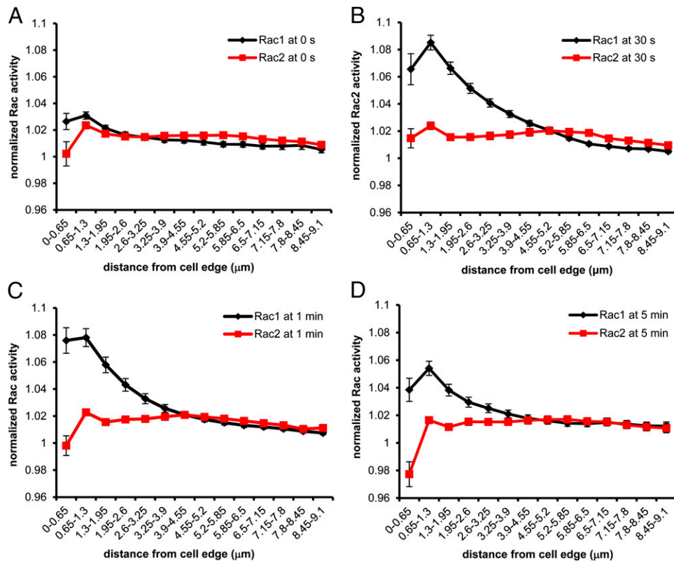
FIGURE 6. Rac1 versus Rac2 activity at the cell periphery during fMLF response. Rac1 and Rac2 activity at the cell edge measured by radial edge-erosion analysis (from Fig. 4C and 5C) overlaid at (A) 0 s, (B) 30 s, (C) 1 min, and (D) 5 min.
