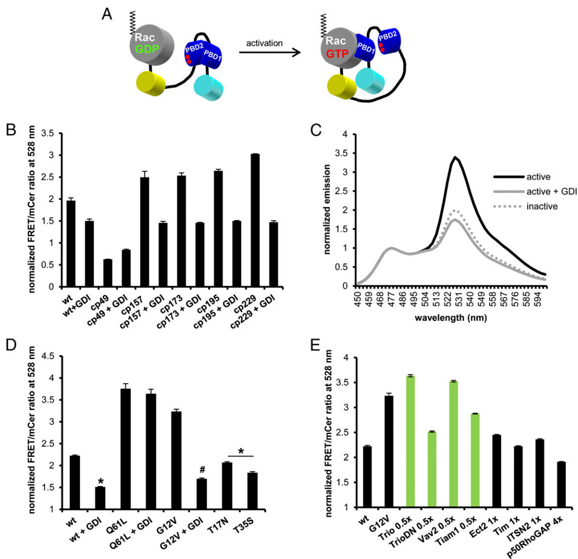
FIGURE 1. Rac1 biosensor optimization. (A) Single-chain Rac biosensor design showing inactive low FRET (left) versus active high FRET states (right). Red dots in PBD2 domain indicate GTPase-binding mutations H83D and H86D. (B) Optimization of WT Rac1 biosensor with circular permutations cp49, cp157, cp173, cp195, and cp229 of mVenus with or without excess GDI. (C) Emission spectra of constitutively active (G12V) with or without excess GDI and dominant negative (T17N) Rac1 biosensor with mcp229Ven, normalized to mCerule1 emission peak at 474 nm. (D) WT or mutant GTPase versions of mcp229Ven Rac1 biosensor in the presence or absence of excess GDI. (E) WT GTPase version of mcp229Ven Rac1 biosensor coexpressed with Rac1-targeting (in green) or nontargeting GEFs (no GDI) and Rac1-targeting p50RhoGAP. Fluorometry data, performed in HEK293 cells, are the mean \pm SEM of three independent experiments performed in triplicate. * p < 0.0001 versus WT alone, # p < 0.00001 versus G12V alone.
