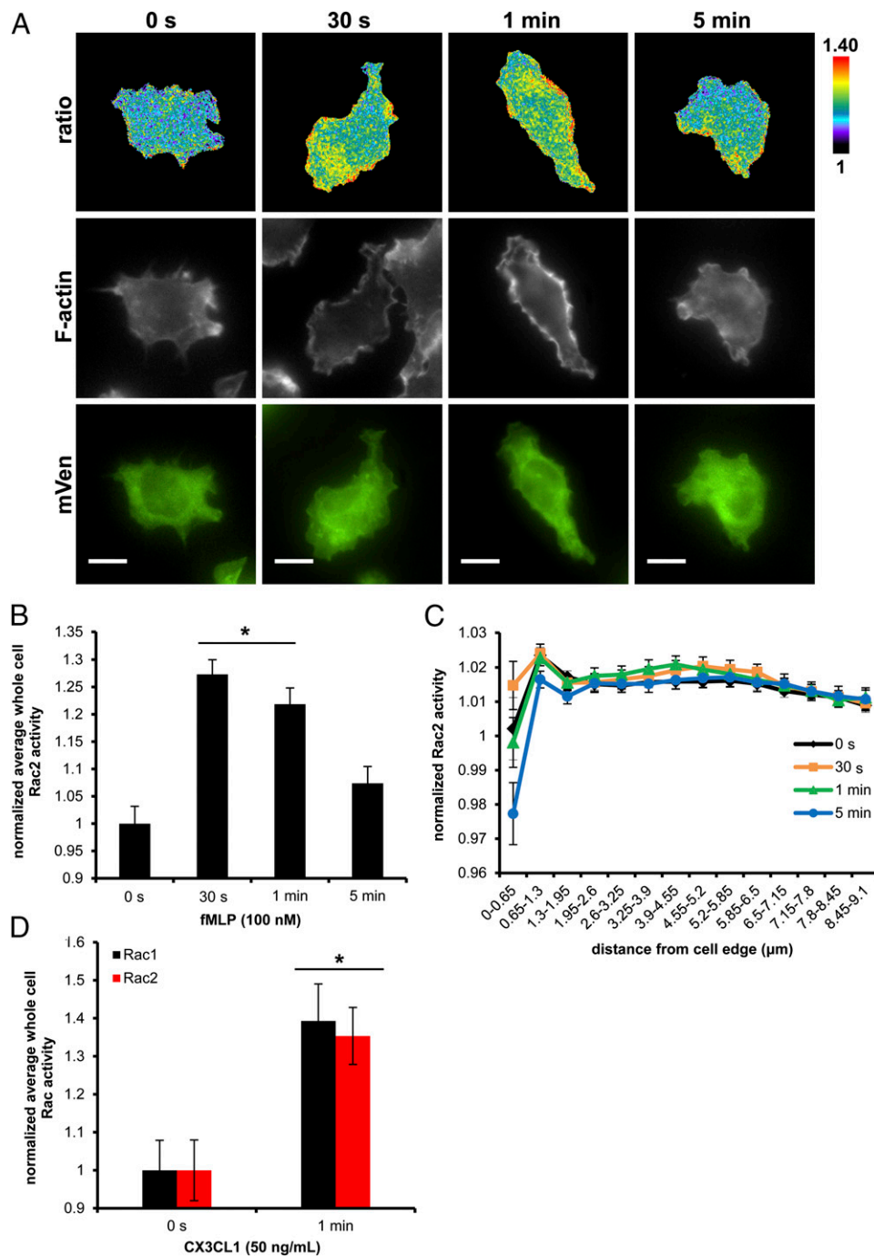
FIGURE 5. Rac2 activation dynamics during fMLF response by macrophages. (A) Representative ratiometric images ( top panel ) of FMLPR.2 cells transiently expressing WT Rac2 biosensor stimulated with 100 nM fMLF for indicated times, stained for F-actin ( middle panel ) and mVen emission to confirm biosensor expression ( bottom panel ). Scale bar, 10 \mu m. (B) Quantitation of whole cell levels of Rac2 activity. *p < 0.0001 versus 0 s. (C) Quantitation of Rac2 activity at the cell edge by radial edge-erosion analysis, where activity was normalized to the lowest value (center region of the cell) within each time point to show relative edge activity. Data are the mean \pm SEM from three independent experiments ( \geq 15 cells per time point per experiment). (D) Quantitation of whole cell levels of Rac1 and Rac2 activity in RAW/LR5 cells transiently expressing Rac1 or Rac2 biosensor and stimulated with 50 ng/ml CX3CL1 for 1 min. Data are mean \pm SEM of n = 12 cells. *p < 0.005 .
