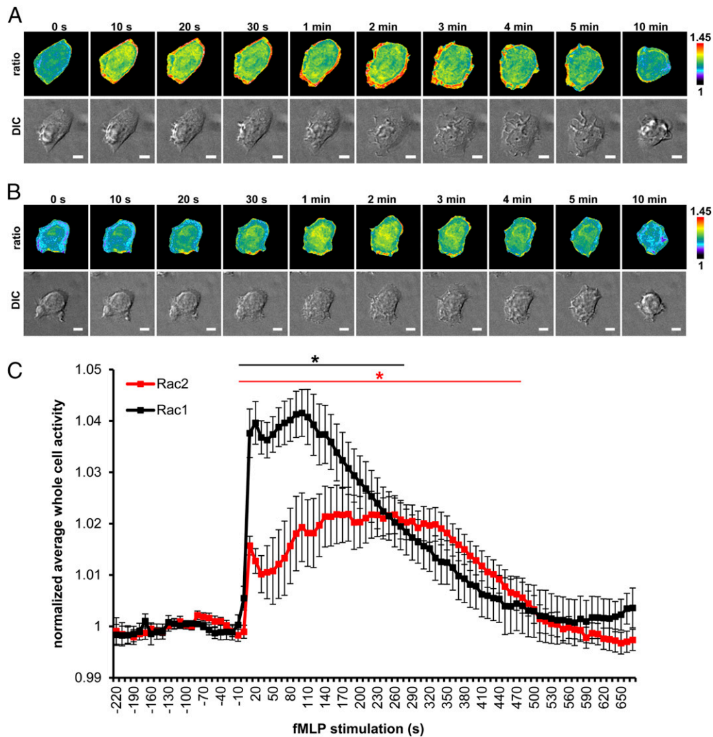
FIGURE 8. Live-cell imaging of Rac1 and Rac2 activation dynamics during fMLF response by macrophages. Time-lapse ratiometric image ( top panel ) and DIC ( bottom panel ) of RAW/LR5 cell line with inducible expression of WT (A) Rac1 and (B) Rac2 biosensor and fMLF-R stably incorporated, stimulated with 100 nM fMLF. Scale bar, 5 \mu m. (C) Quantitation of whole cell levels of Rac1 and Rac2 activity, normalized to average whole cell activity before stimulation (baseline activity during the first 4 min prior to stimulation). Statistical significance was determined using one-tailed, paired student t test. Data are the mean \pm SEM of 11 cells for Rac1 and 10 cells for Rac2. Black asterisk, *p < 0.05 , 10–270 s versus 0 s (Rac1). Red asterisk, *p < 0.05 , 10–480 s versus 0 s (Rac2).
