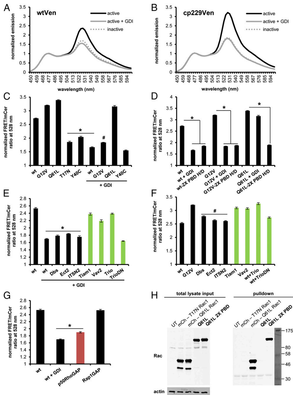
FIGURE 2. Characterization of new Rac2 biosensor. Normalized emission spectra of constitutively active (G12V) with or without excess GDI and dominant negative (T17N) Rac2 sensor containing (A) original mVen (B) mcp229Ven, normalized to mCerule1 donor emission peak at 474 nm. (C) WT or mutant GTPase versions of mcp229Ven Rac2 biosensor in the presence or absence of excess GDI. (D) WT and mutant versions of Rac2 biosensor with or without the GTPase-binding deficient H83D and H86D mutations in PBD1 (2× PBD H/D = both PBD1 and PBD2 are GTPase-binding deficient) in the presence or absence of excess GDI. (E) WT GTPase version of mcp229Ven biosensor coexpressed with Rac2-targeting (in green) or nontargeting GEFs in the presence or (F) absence of excess GDI. (G) WT GTPase version of mcp229Ven biosensor coexpressed with excess of targeting (in red) or nontargeting GAPs. (H) Western blot of GST-PAK pull-down of mCherry-tagged Q16L and T17N Rac1 for assay control, and Q61L constitutively active version of the Rac2 biosensor with functional or GTPase-binding-deficient mutations in the PBD1 domain, overexpressed in HEK293 cells. Total lysates and actin was used as a loading control. Fluorometry data, performed in HEK293 cells, are the mean \pm SEM of three independent experiments performed in triplicate. * p < 0.00001 versus WT alone, # p < 0.00001 versus G12V alone.
