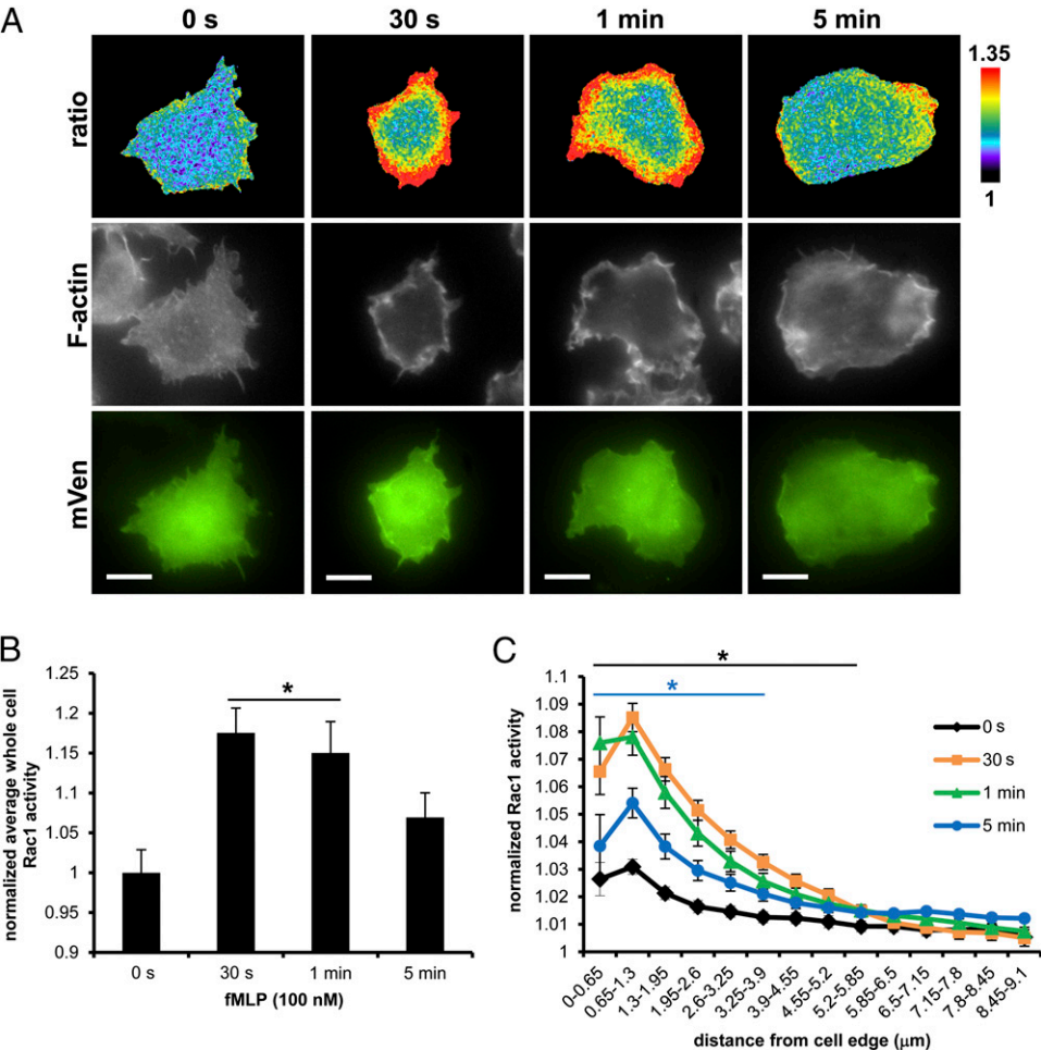
FIGURE 4. Rac1 activation dynamics during fMLF response by macrophages. (A) Representative ratiometric images (top panel) of FMLPR.2 cells transiently expressing WT Rac1 biosensor stimulated with 100 nM fMLF for indicated times before fixation, stained for F-actin (middle panel) and mVen emission to confirm biosensor expression (bottom panel). Scale bar, 10 \mu m. (B) Quantitation of whole cell levels of Rac1 activity. ^*p < 0.0001 versus 0 s. (C) Quantitation of Rac1 activity at the cell edge by radial edge-erosion analysis, where activity was normalized to the lowest value (center region of the cell) within each time point to show changes in relative edge activity. Data are the mean \pm SEM from three independent experiments ( \geq 15 cells per time point per experiment). Black asterisk, ^*p < 0.0001 for 30 s and 1 min versus 0 s in 0–5.85- \mu m region. Blue asterisk, ^*p < 0.02 for 5 min versus 0 s in 0–3.9 \mu m.
