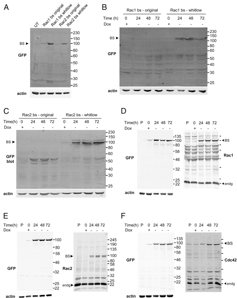
FIGURE 7. Optimization of biosensor expression in macrophages. Western blot analysis of (A) original (nonoptimized) or whitlow-modified Rac1 and Rac2 biosensors transiently expressed overnight. (B) Tet-OFF inducible expression of original or whitlow-modified Rac1 and (C) Rac2 biosensor. (D) Tet-OFF induction of fully optimized, FACS-sorted Rac1, (E) Rac2, and (F) Cdc42 biosensors. BS, biosensor; Dox, doxycycline at 2 \mu\text{g/ml} ; endg, endogenous; P, untransduced parental RAW/LR5 lysate; UT, untransfected.
