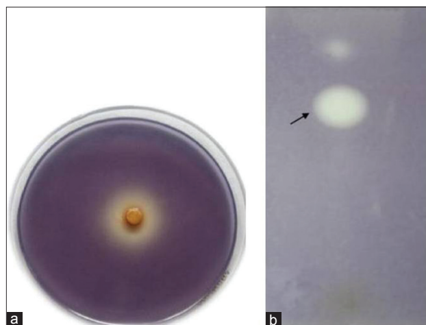
Figure 1: Anti-QS activity of active fraction (AEF) of A. pavonina . (a) Biosensor bioassay of AEF showing inhibition of C 6 -AHL-mediated violacein production in bioreporter C. violaceum CV026 (b) TLC overlay assay of AEF illustrating the inhibition of C 6 -AHL-mediated violacein production in C. violaceum CV026. Areas of pigment clearing (indicated by arrow) show region of AEF compounds that inhibit AHL-regulated violacein production in C. violaceum CV026
