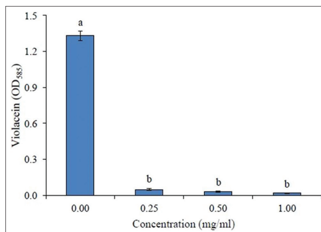
Figure 2: Inhibition of violacein production in C. violaceum ATCC12472 by different concentrations of active fraction (AEF) of A. pavonina . Values are expressed as mean \pm SD, n = 4 . Same letters in the columns (bar) are not significantly different ( P < 0.001 )
