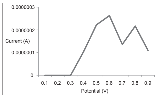
Figure 2: Oxidation current of \text{H}_2\text{O}_2 at many potentials using Pt electrode
